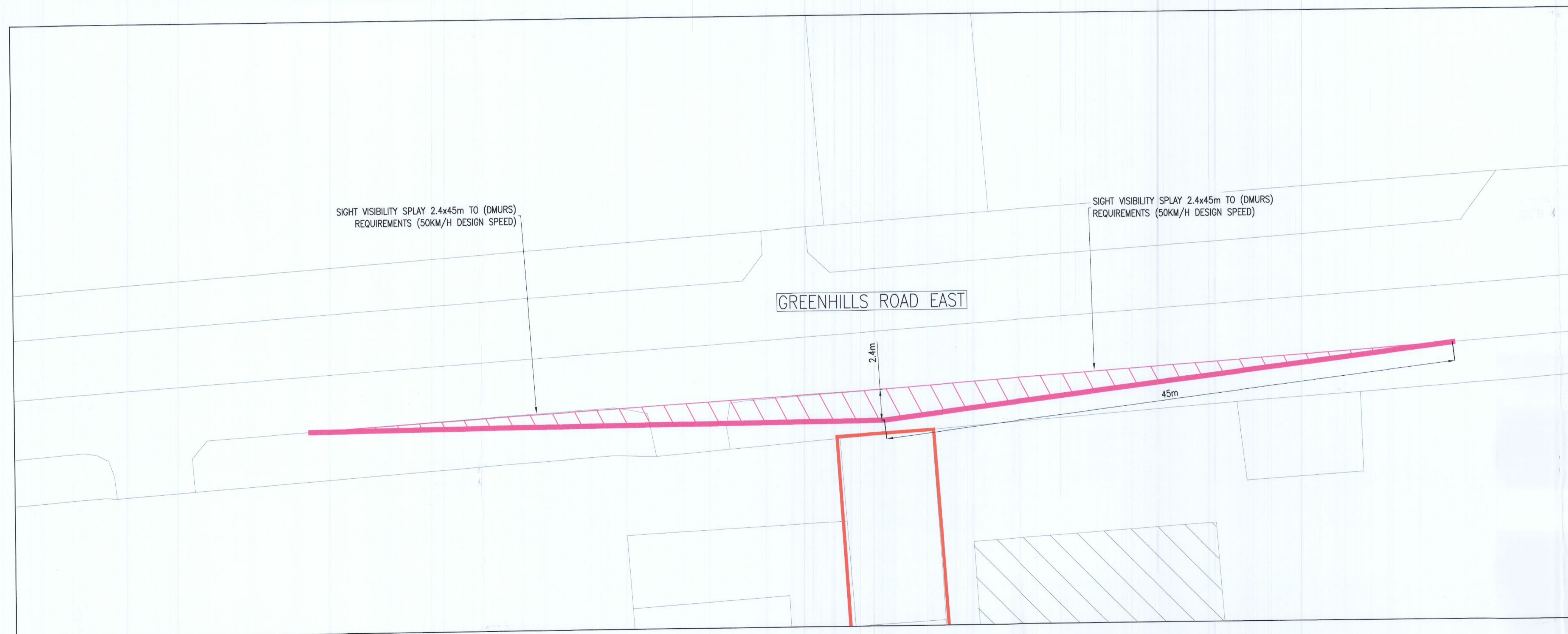
EASTERN EXIT SCALE 1:200
