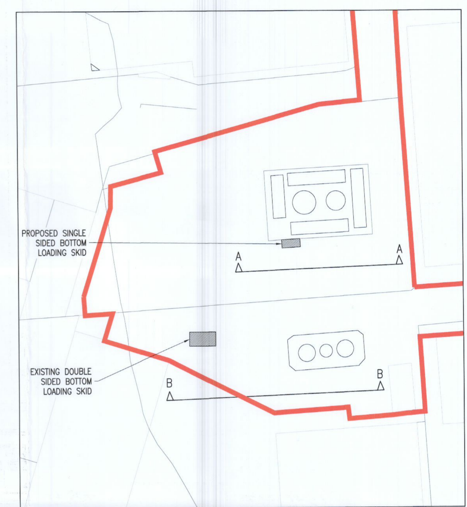
KEYPLAN SCALE 1:500
