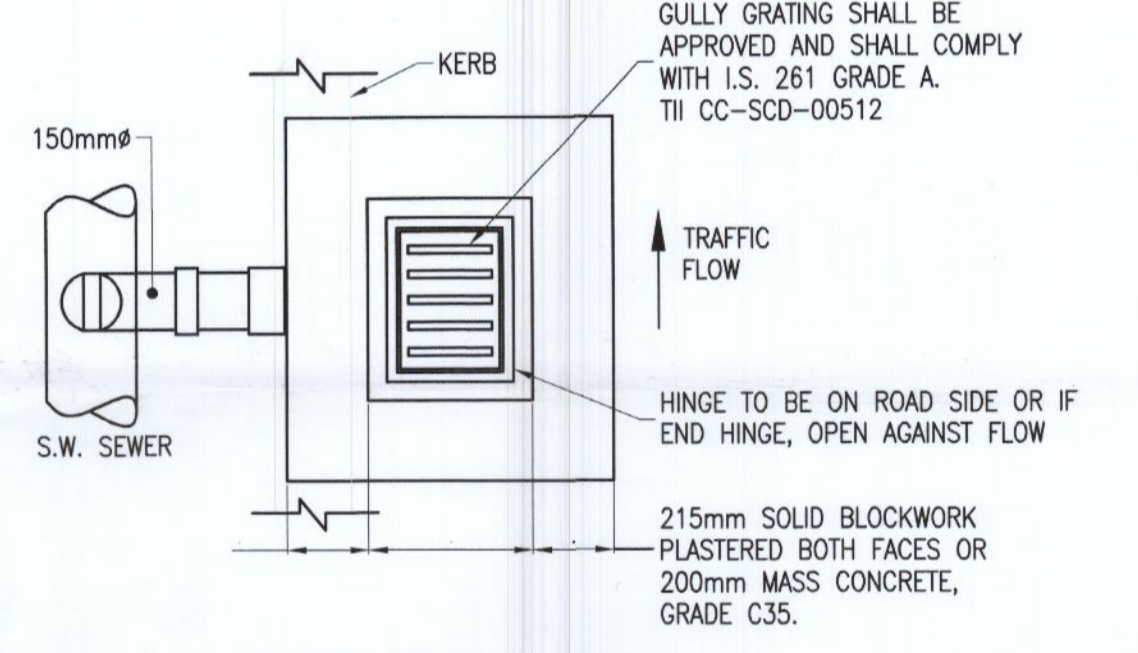
PLAN OF ROAD GULLY (TII CC-SCD-00511) SCALE 1:20
