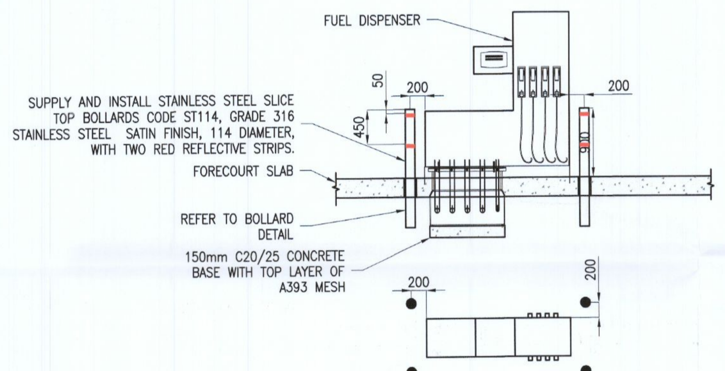
RETAIL FORECOURT PUMP DETAIL SCALE 1:50
