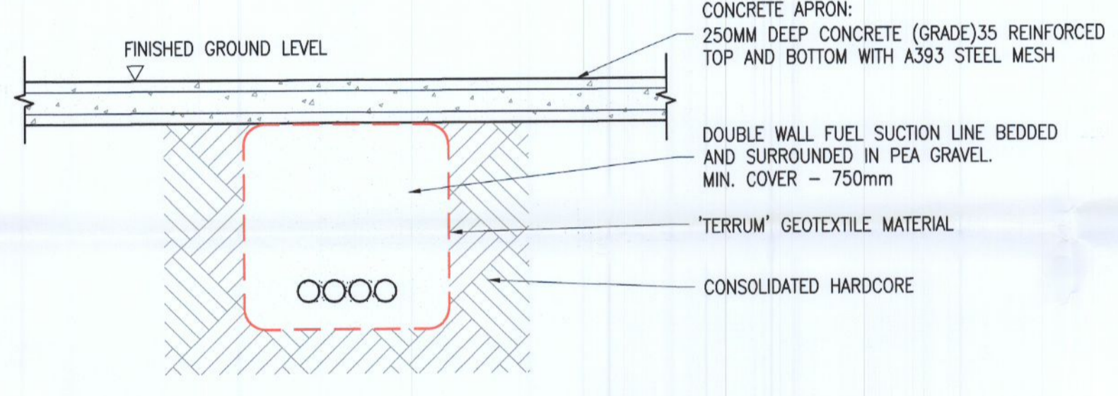
FUEL PIPEWORK SECTION SCALE 1:25
