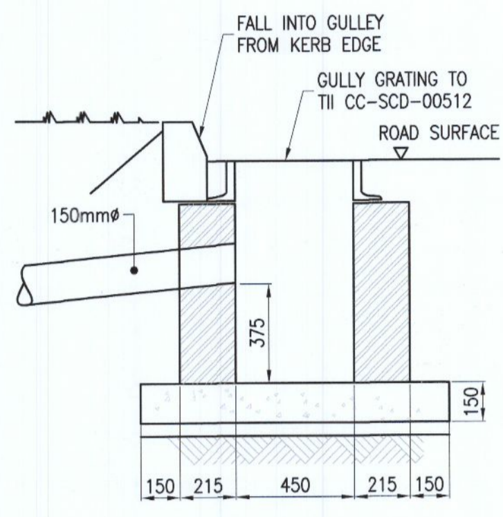
SECTION THROUGH ROAD INLET GULLY (TII CC-SCD-00511) SCALE 1:20
