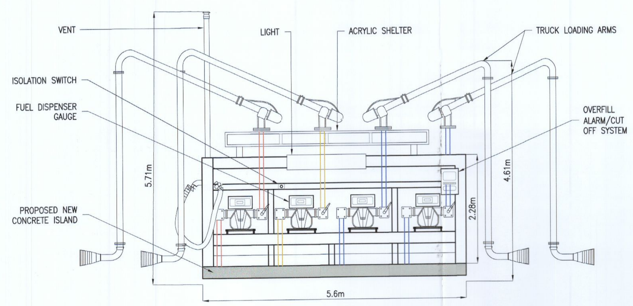
PROPOSED BOTTOM LOADING SKID FRONT ELEVATION SCALE 1:50
