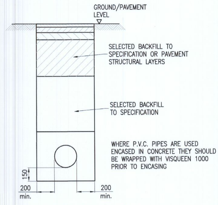
GRANULAR SURROUND DETAIL FOR SEWERS AND DRAINS (TII CC-SCD-00521-TYPE S) SCALE 1:20
