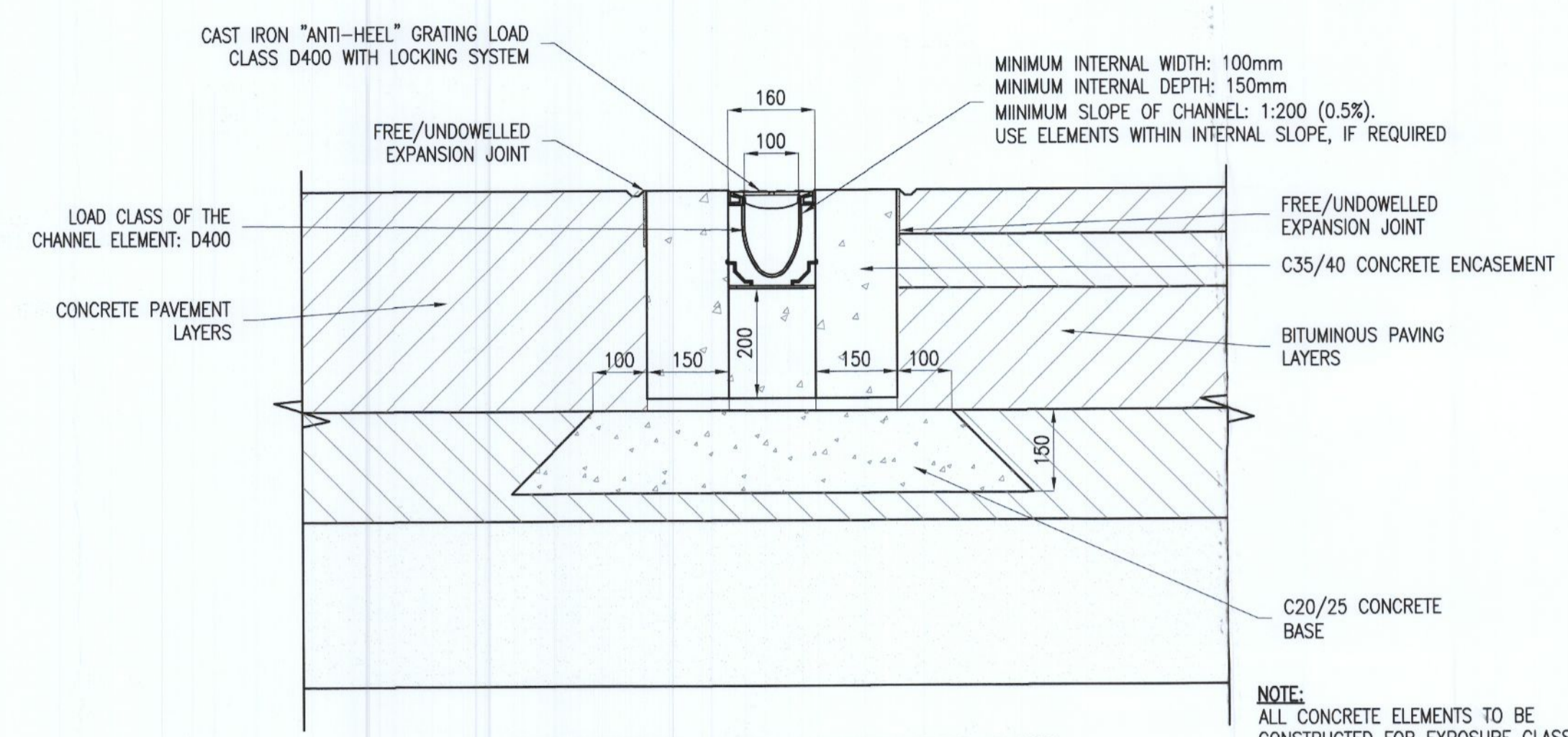
TYPICAL SECTION THROUGH FORECOURT LINEAR CHANNEL DRAIN (ACO DRAIN OR SIMILAR) SCALE 1:10
