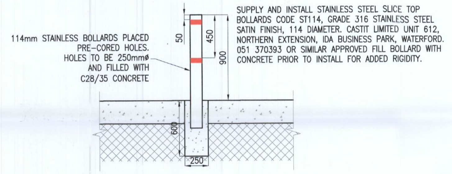
STAINLESS STEEL BOLLARD DETAIL SCALE 1:25
