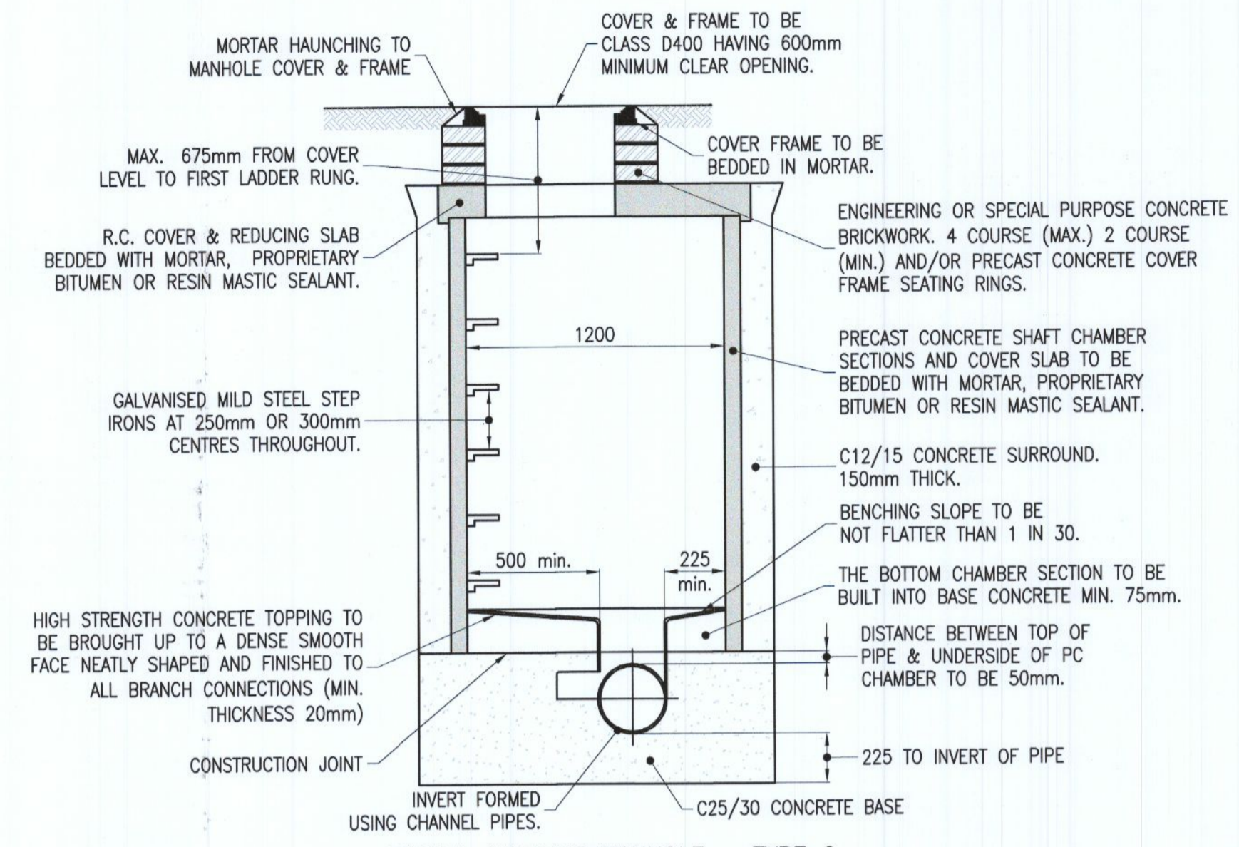
TYPICAL PRECAST MANHOLE - TYPE C (TII CC-SCD-00504) SCALE 1:25
