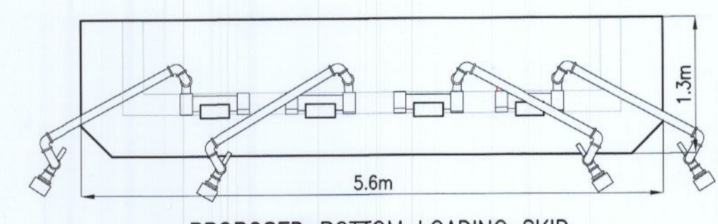
PROPOSED BOTTOM LOADING SKID PLAN SCALE 1:50
