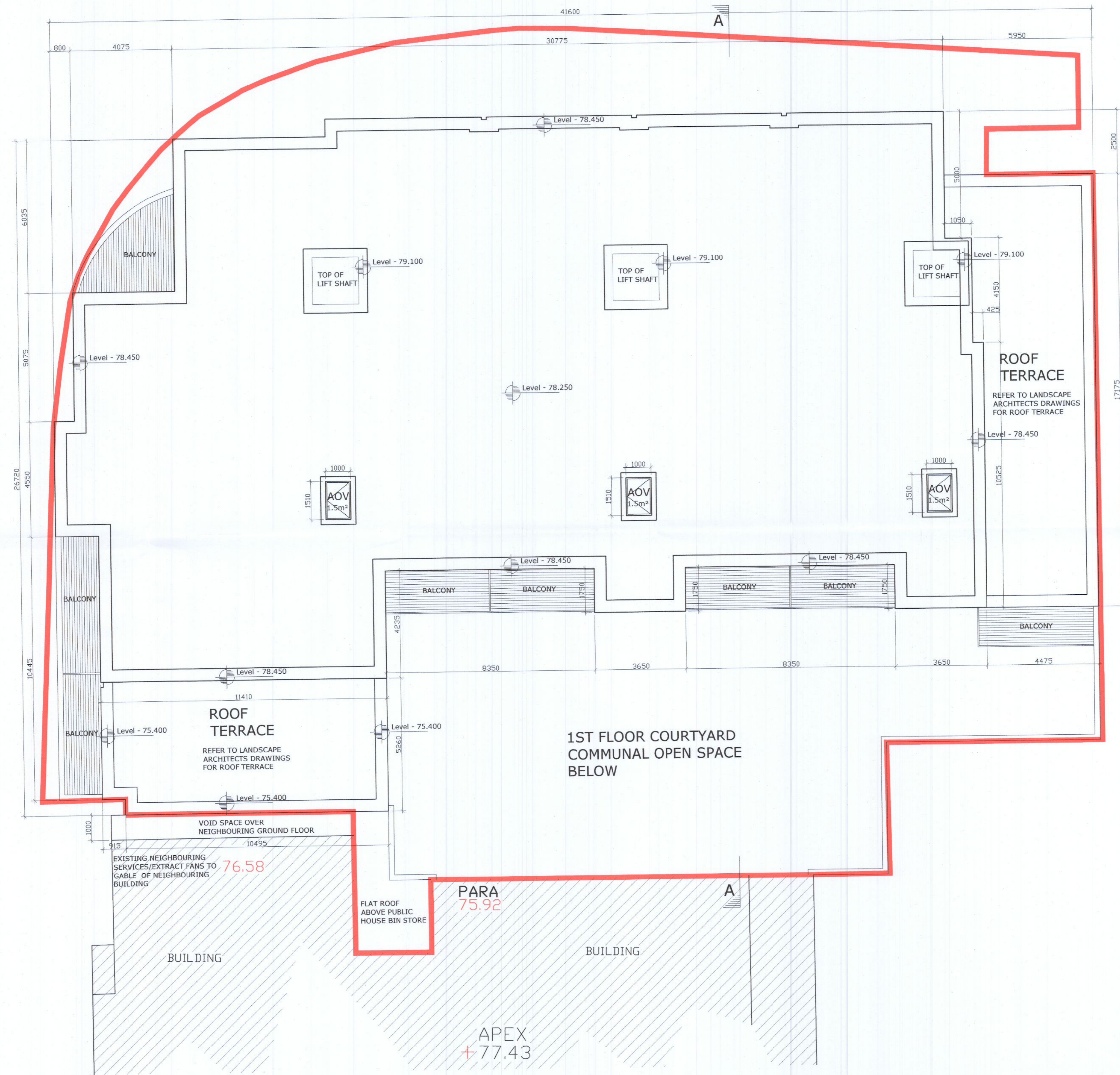
Proposed Roof Plan Scale 1:100
