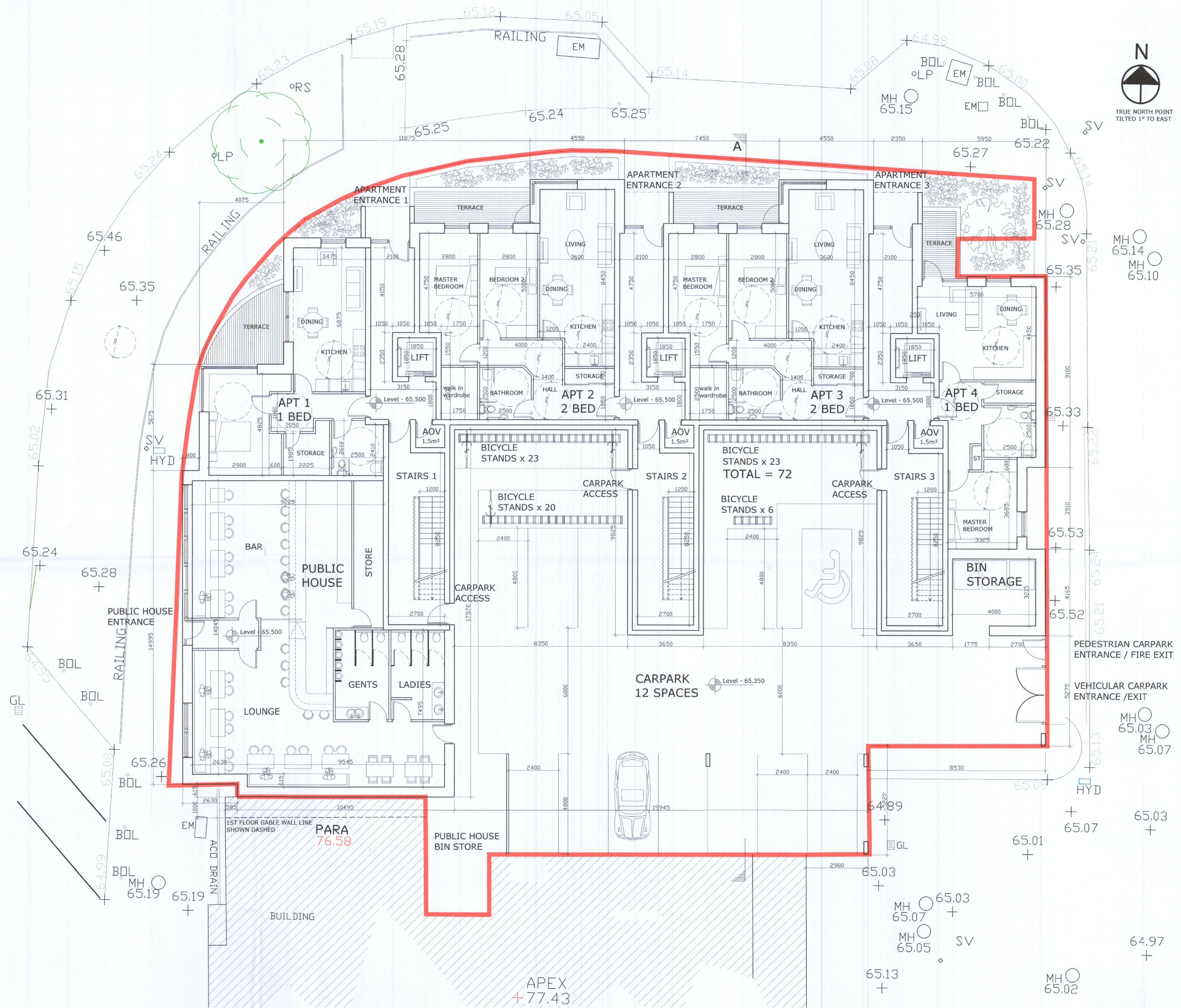
Proposed Ground Floor Plan Scale 1:100 A1, 1:200 A3
