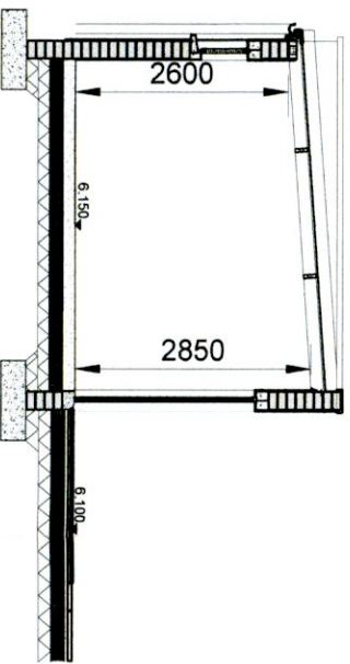
SECTION SCALE 1:100
