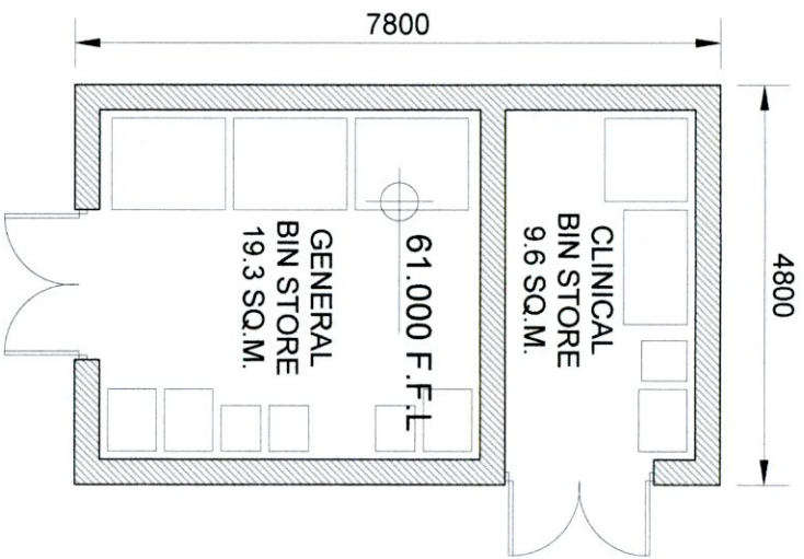
PROPOSED PLAN SCALE 1:100
