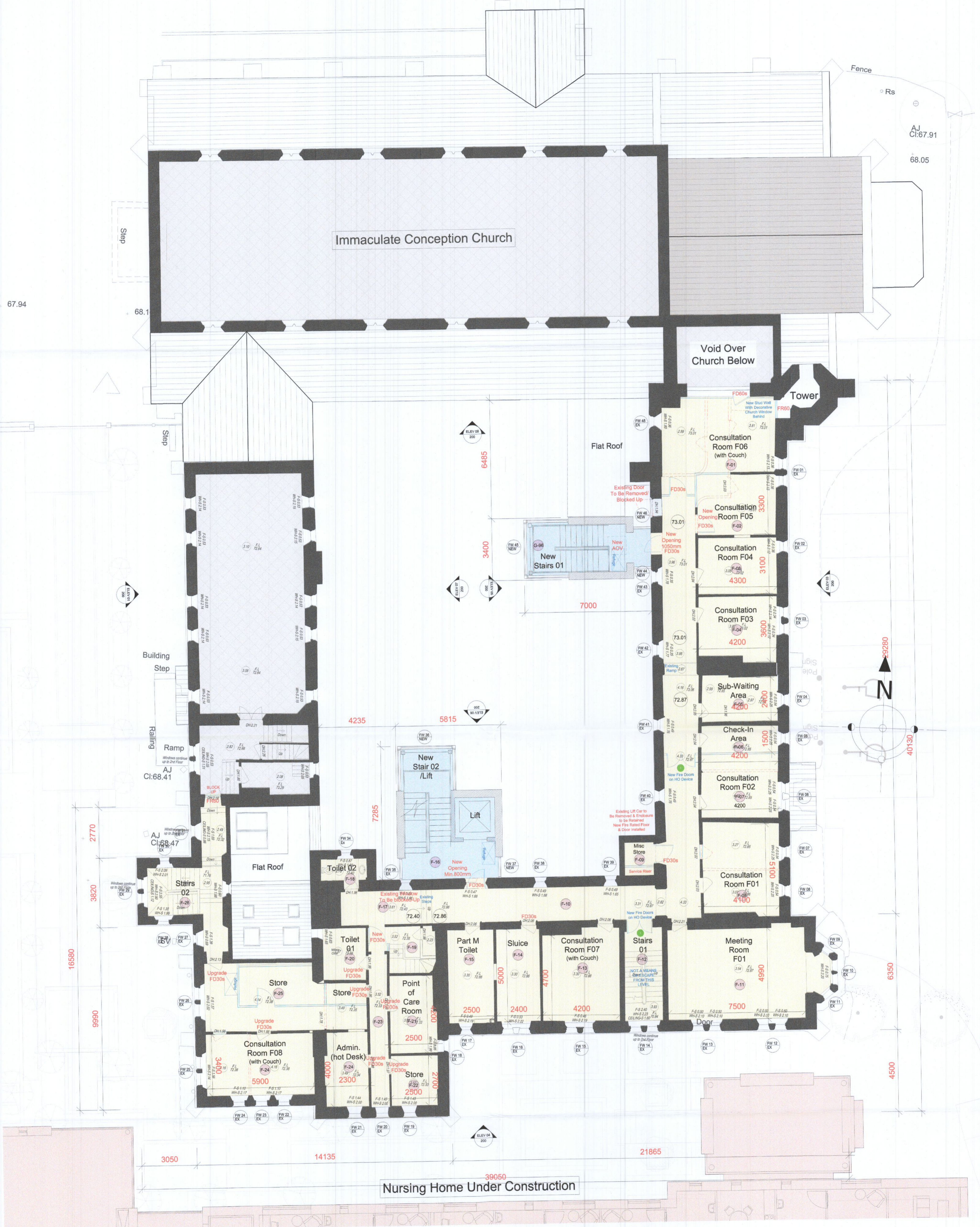
PROPOSED FIRST FLOOR PLAN
