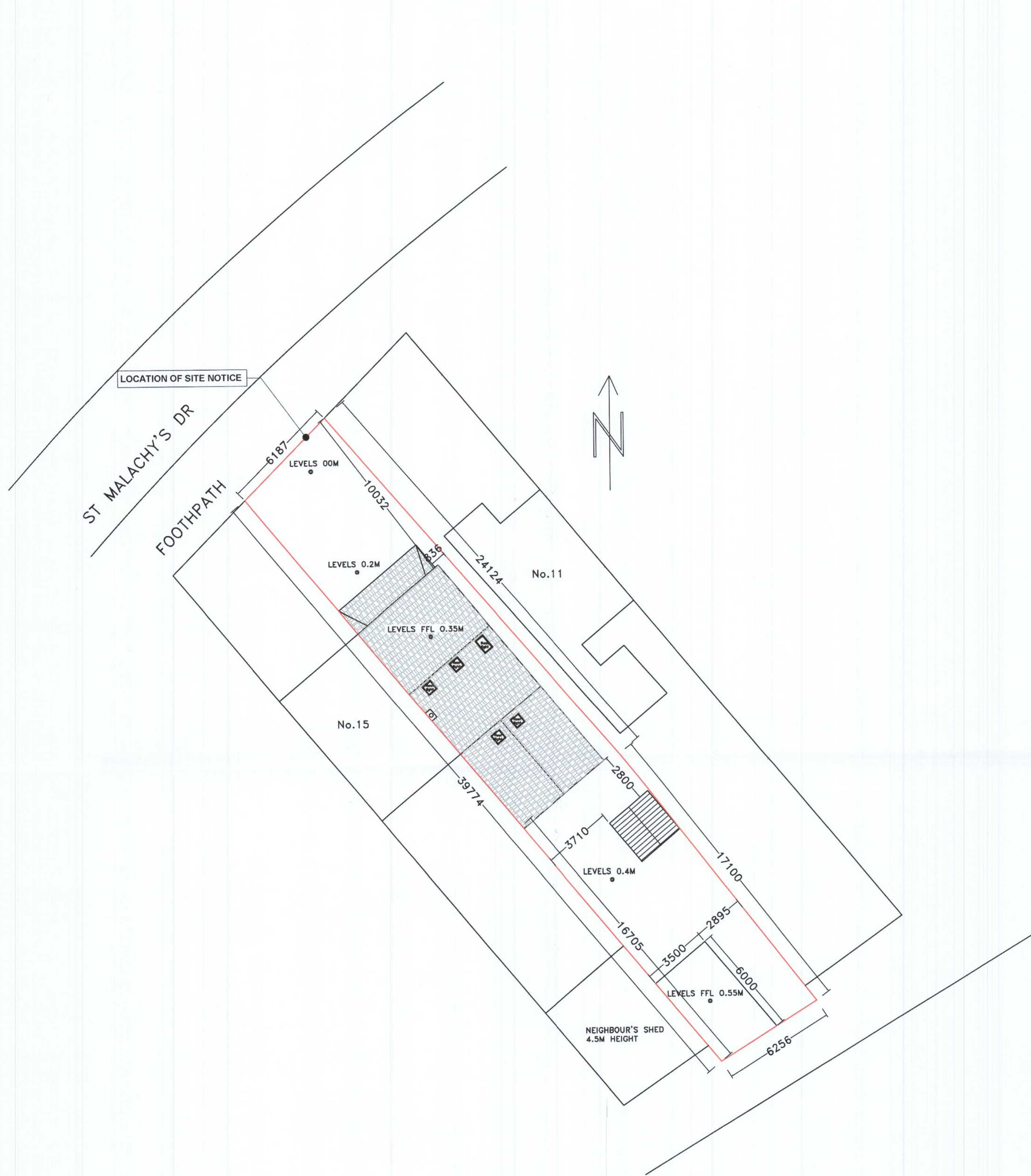
SITE LAYOUT PLAN (EXISTING) SCALE 1:150
