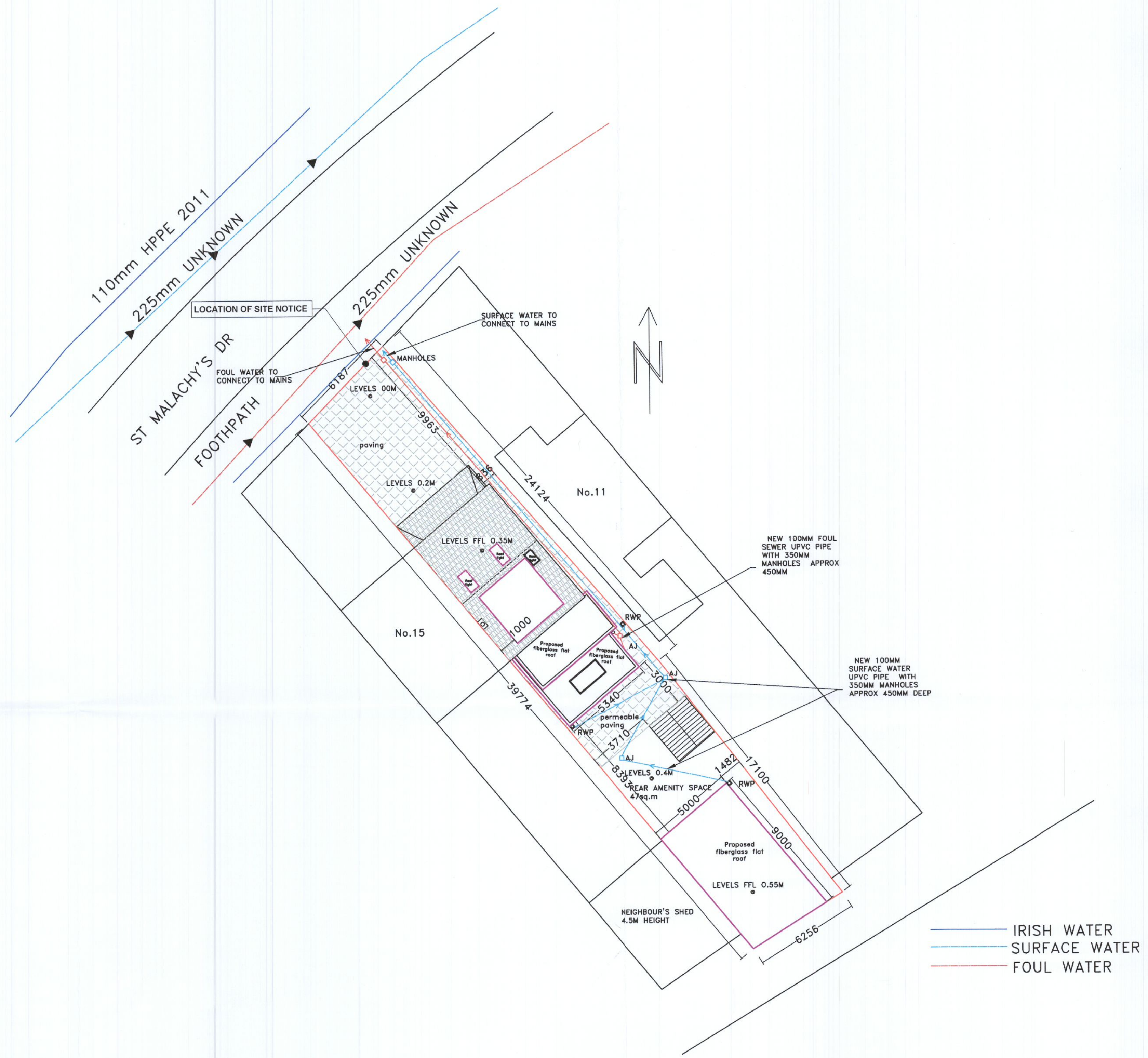
SITE LAYOUT PLAN (PROPOSED) SCALE 1:150
