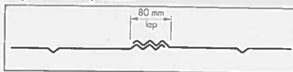
Figure 4 Overlap details
