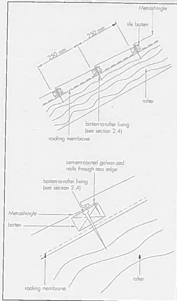
Figure 3 Spacing and fixing detail
