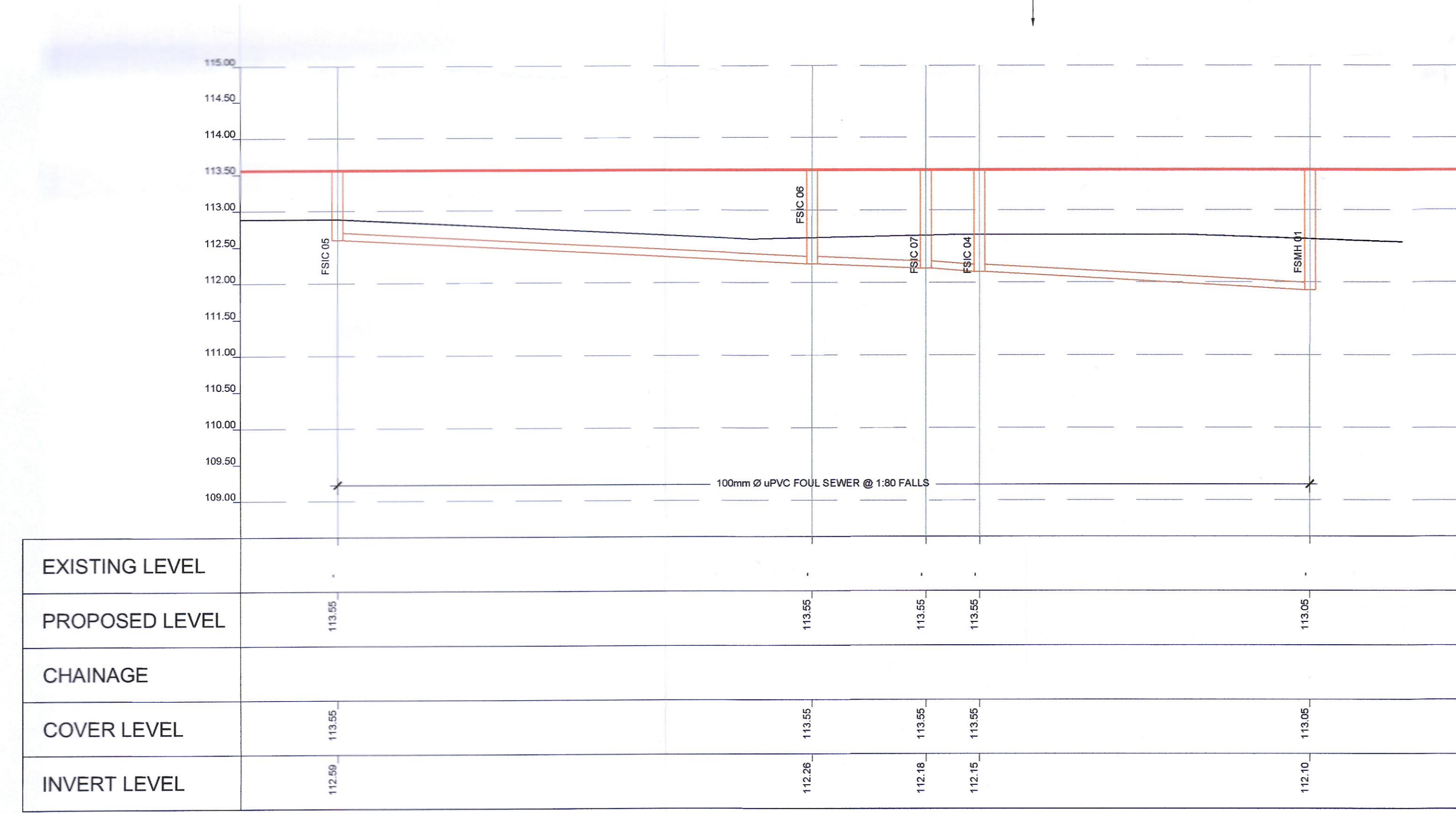
2 VERTICAL SECTION FSIC 05 TO FSMH 01 HORIZONTAL SCALE 1:200 VERTICAL SCALE 1:50
