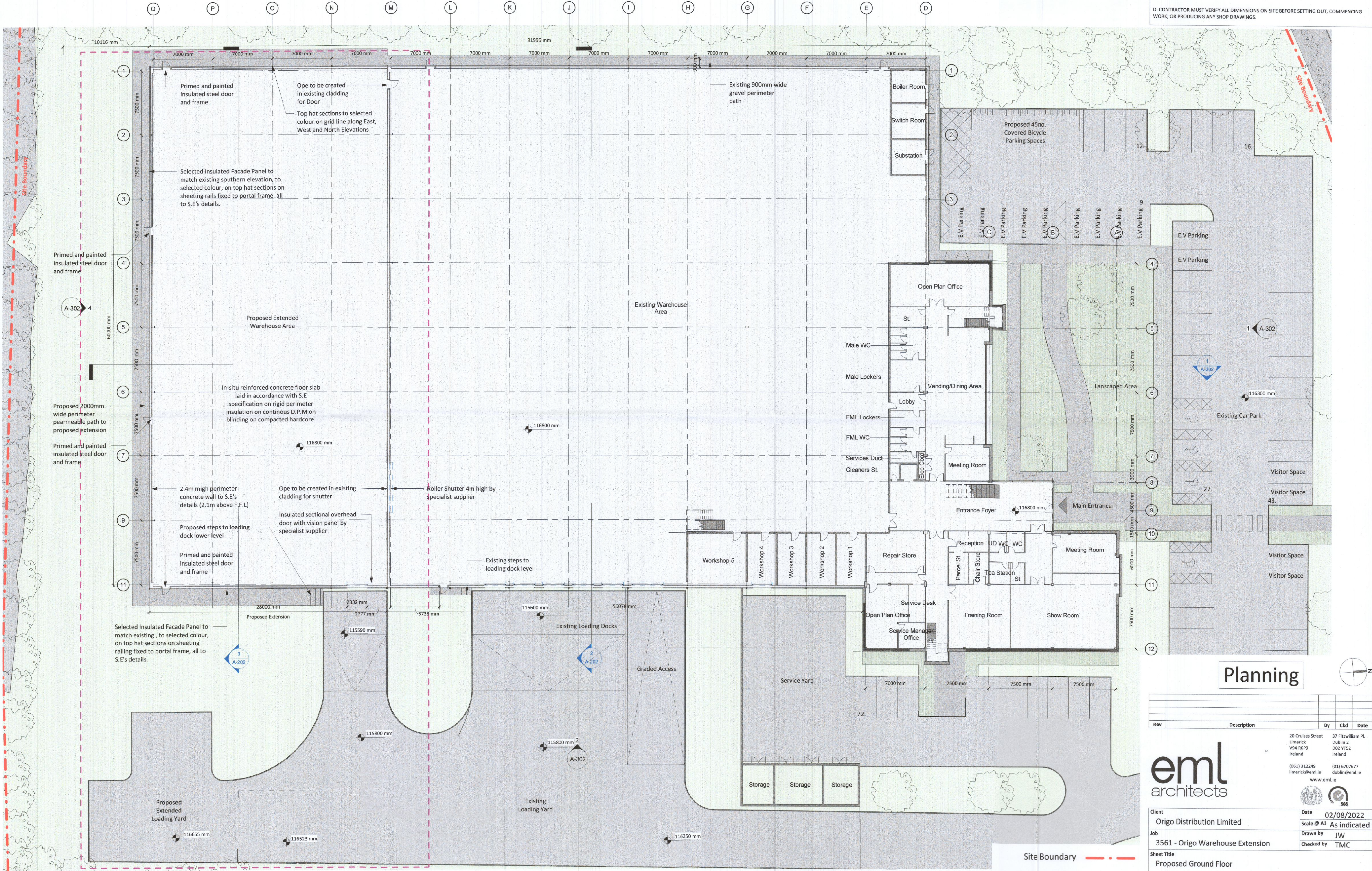
1 00 - Proposed Ground Floor 1 : 200
