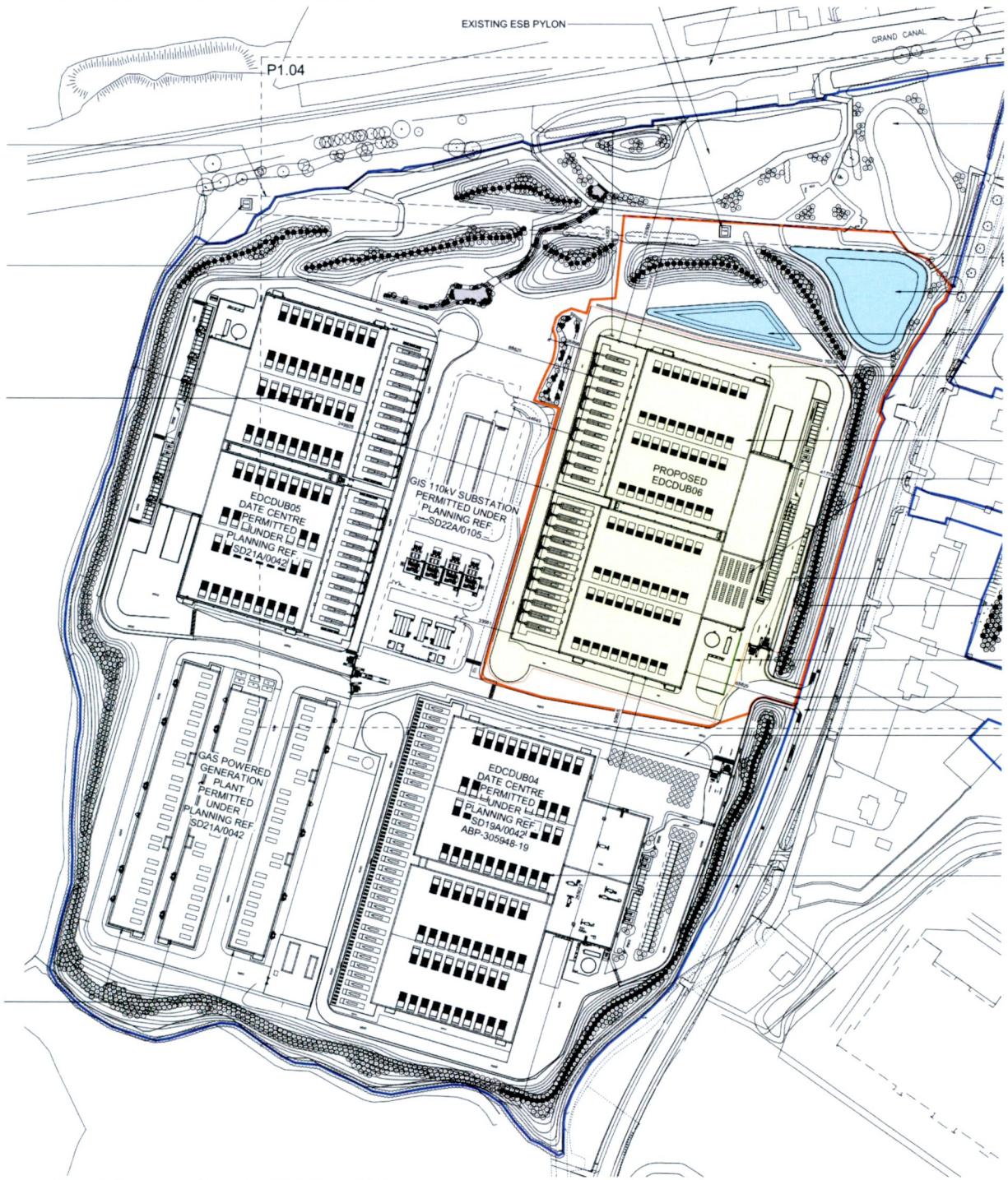
Figure 1 Proposed site layout plan
