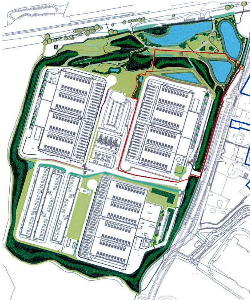
Fig 01 – Landscape Masterplan
