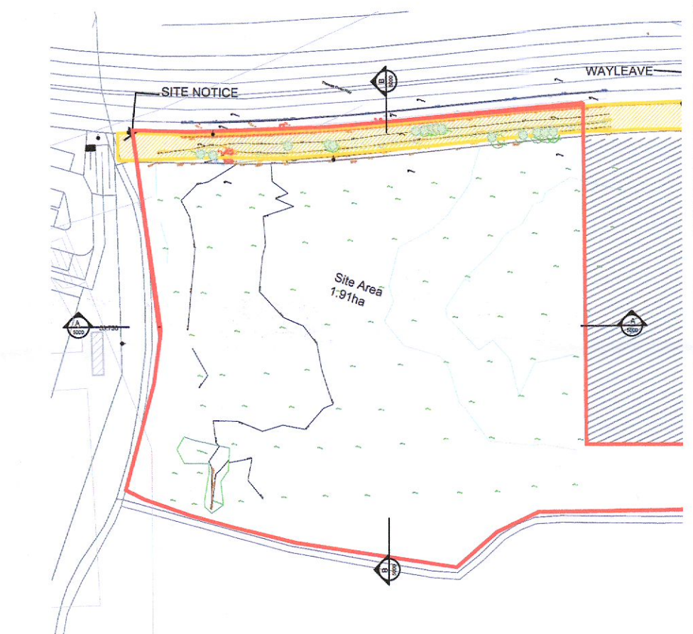
03 5000 EXISTING SITE KEY PLAN 1:1500 @ A1
