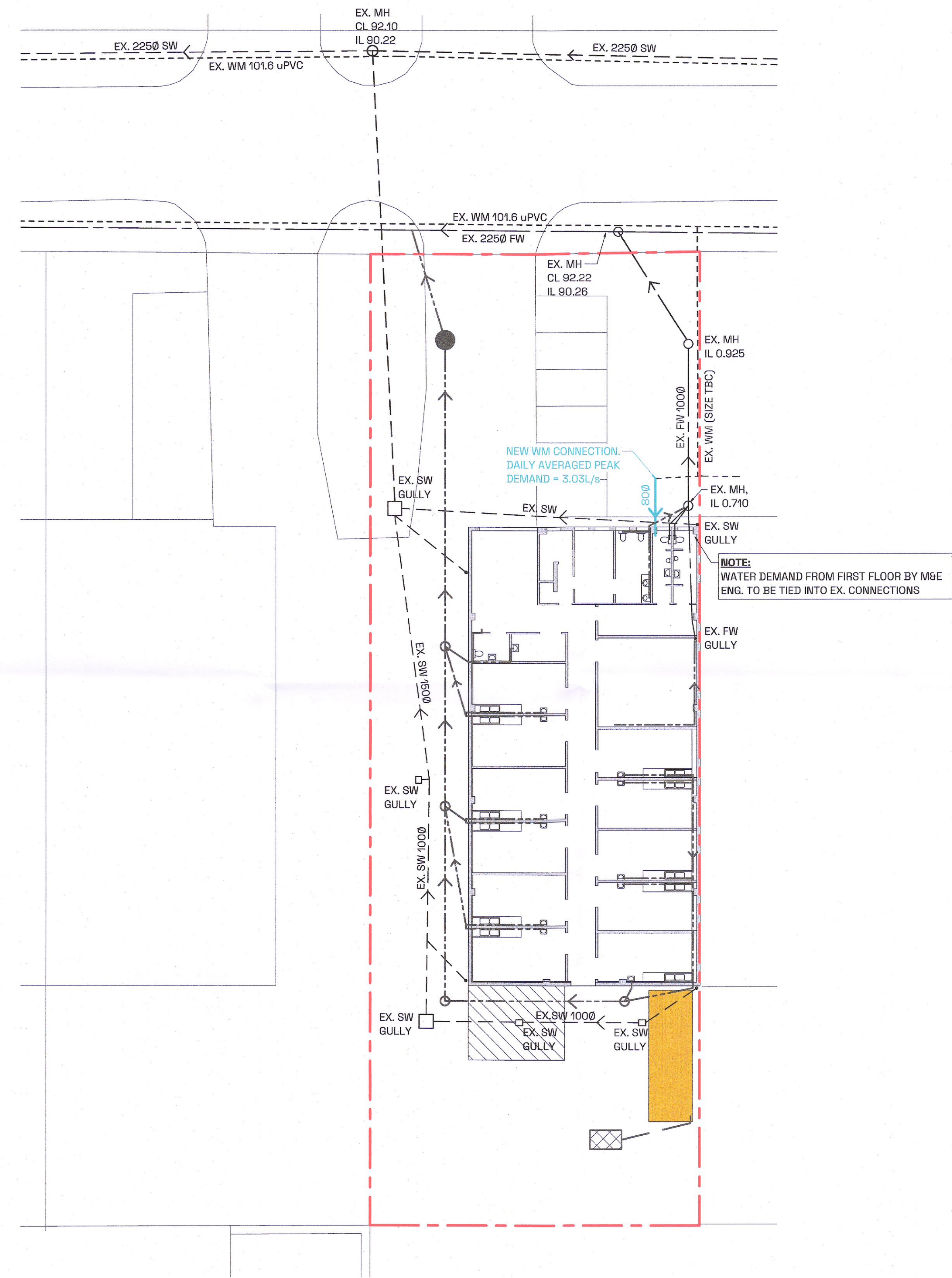
PROPOSED WATERMAIN LAYOUT 1:200
