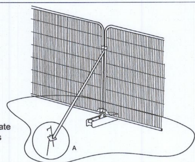
Stabilizer struts installed on every fencing panel section on the tree protection side
