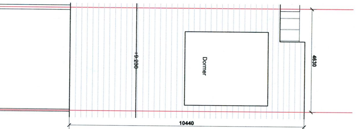
Proposed Roof Plan Scale - 1:100
