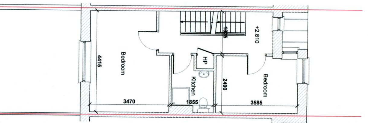
Proposed First Floor Plan Scale - 1:100 (No Change)
