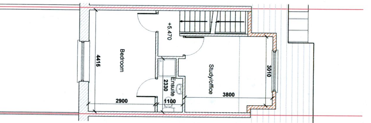
Proposed Second Floor Plan Scale - 1:100
