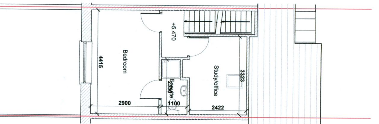
Existing Second Floor Plan Scale - 1:100
