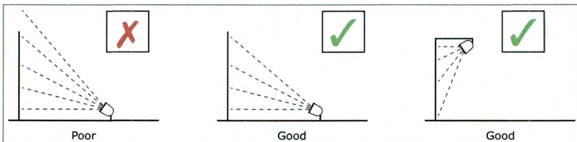
Figure 4: Façade illumination
