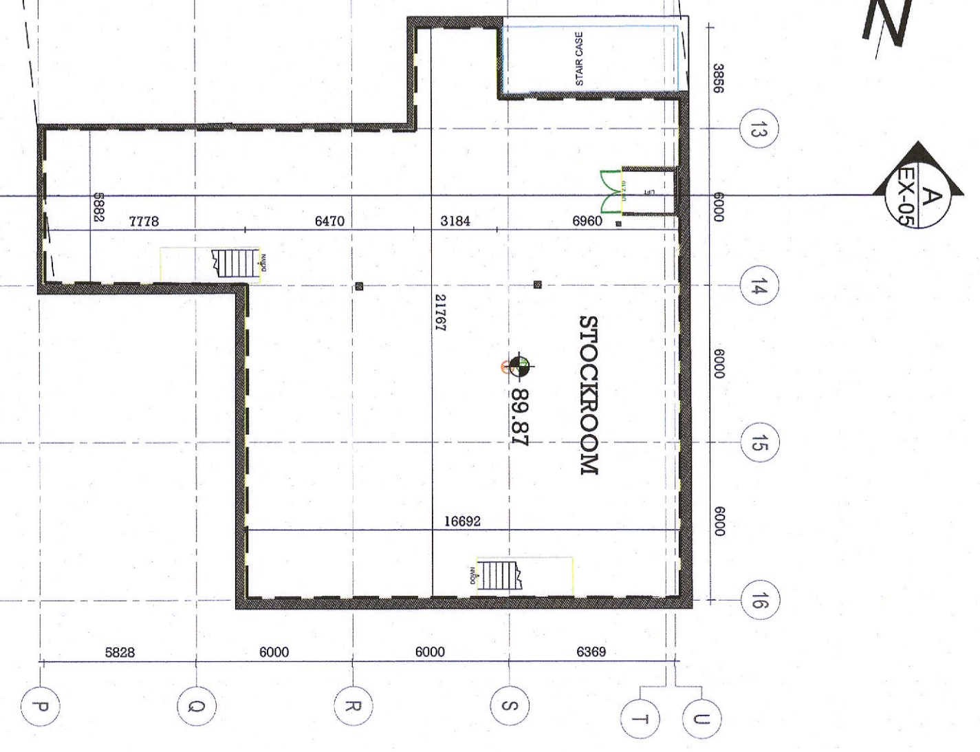
EXISTING MEZZANINE FLOOR PLAN - STOCKROOM 3 SCALE: 1:200 @ A1
