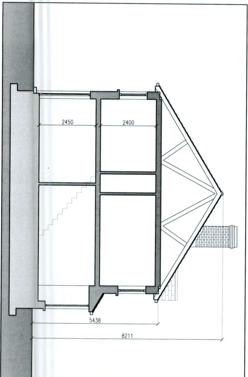
Existing Diagrammatic Section
