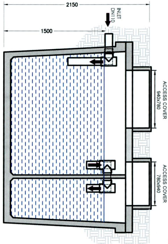
SECTION B-B
