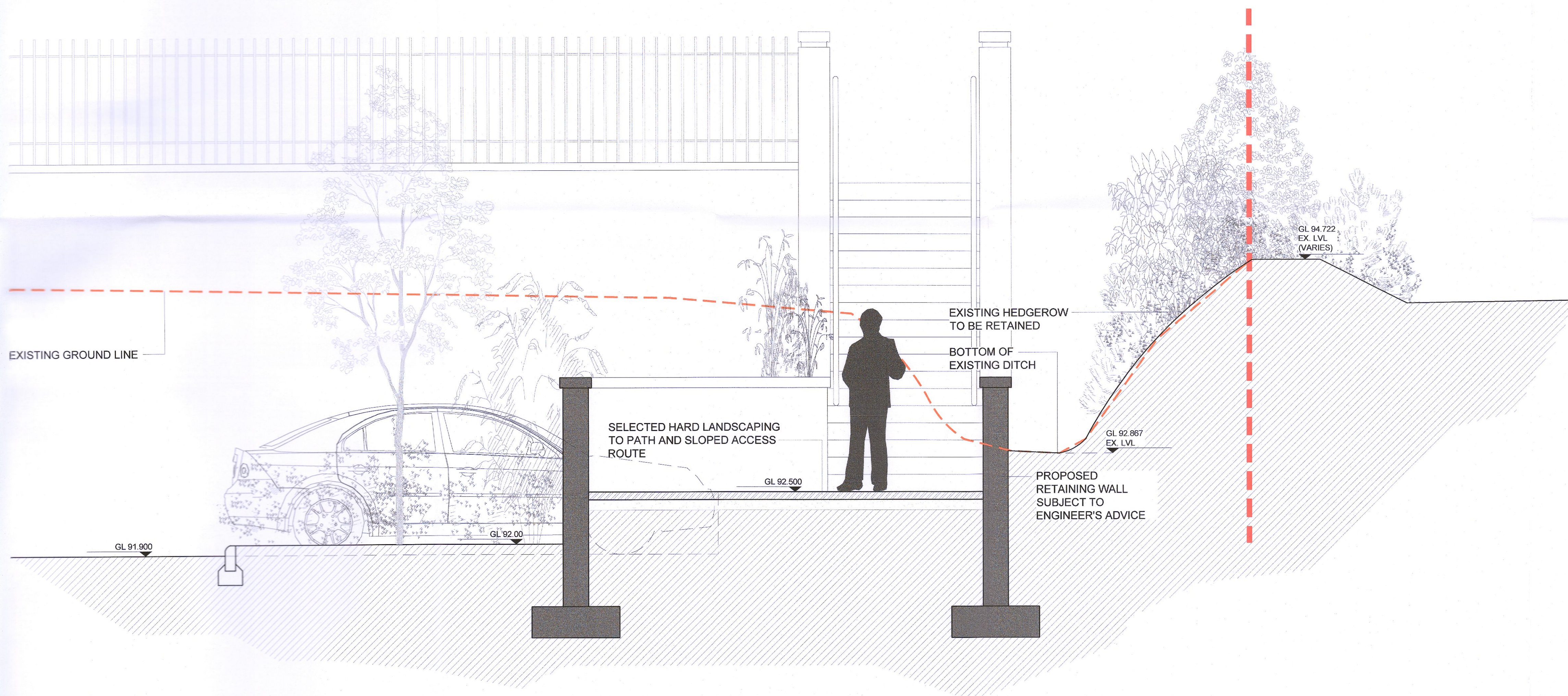
01 Proposed Boundary Wall (Boundaries F-G) Section PA 502 1:25
