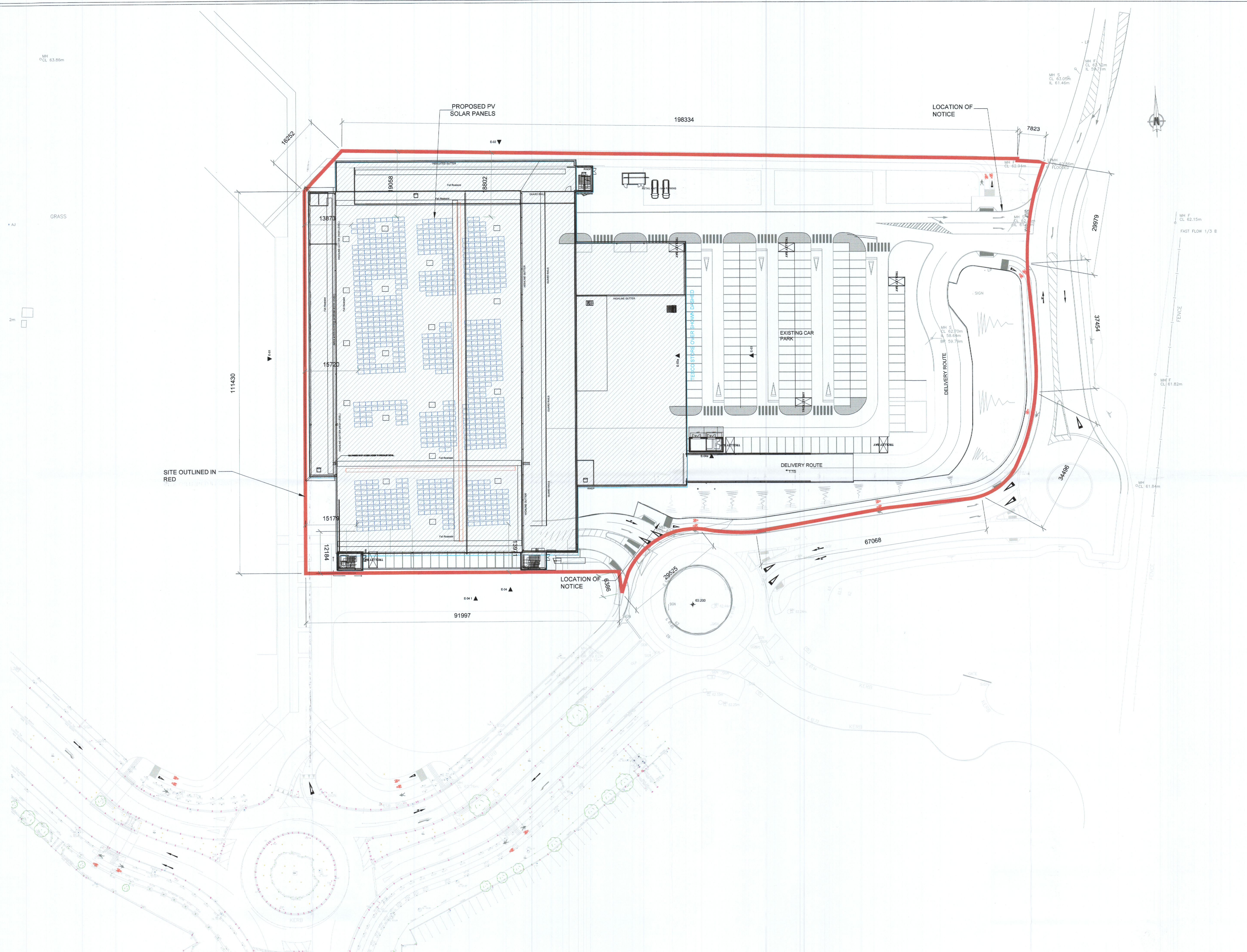
SOLAR PANEL ARRANGEMENT SITE LAYOUT PLAN VIEW SCALE 1:500
