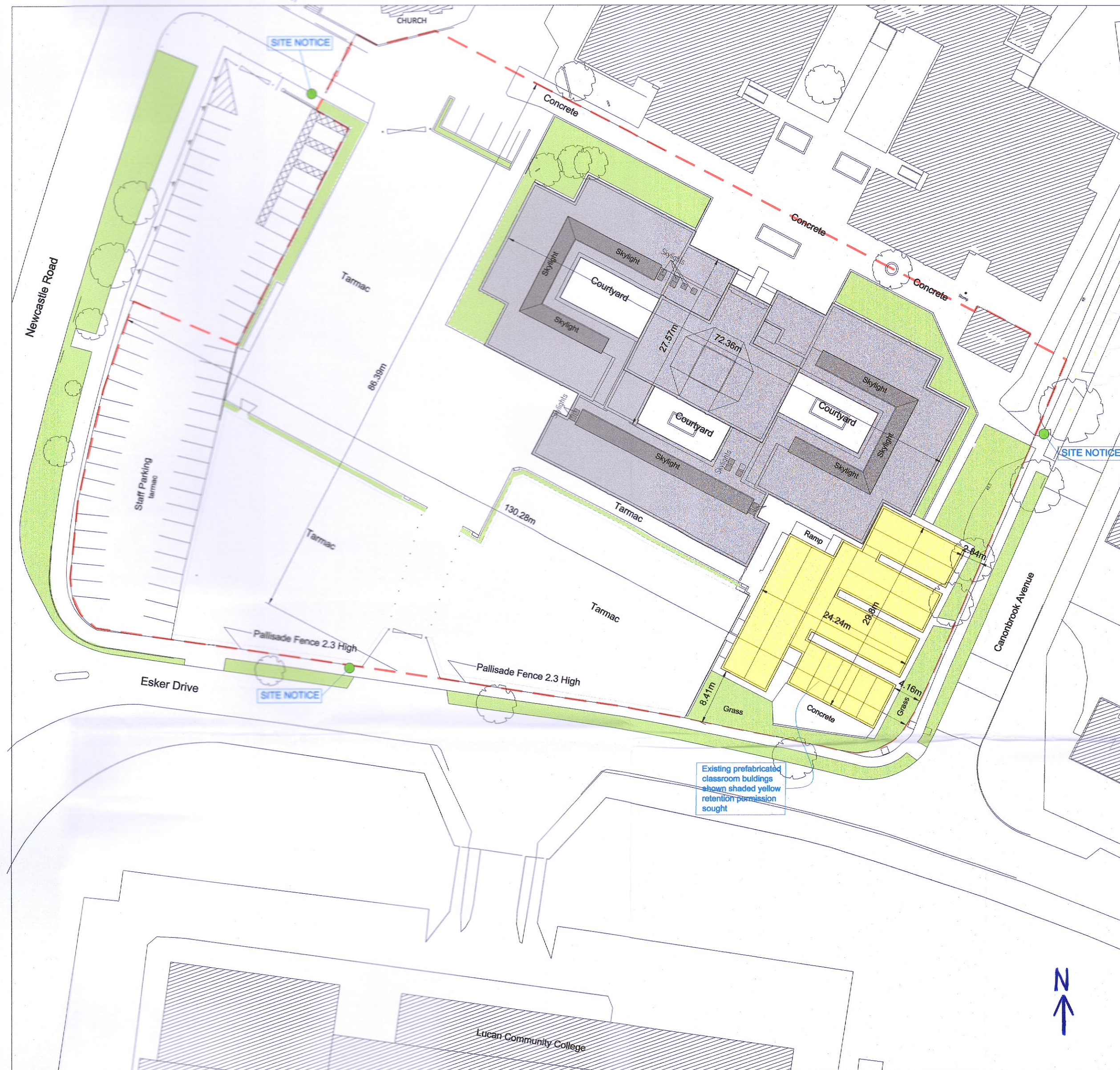
EXISTING SITE LAYOUT (BLOCK PLAN) scale: 1:500@ A1
