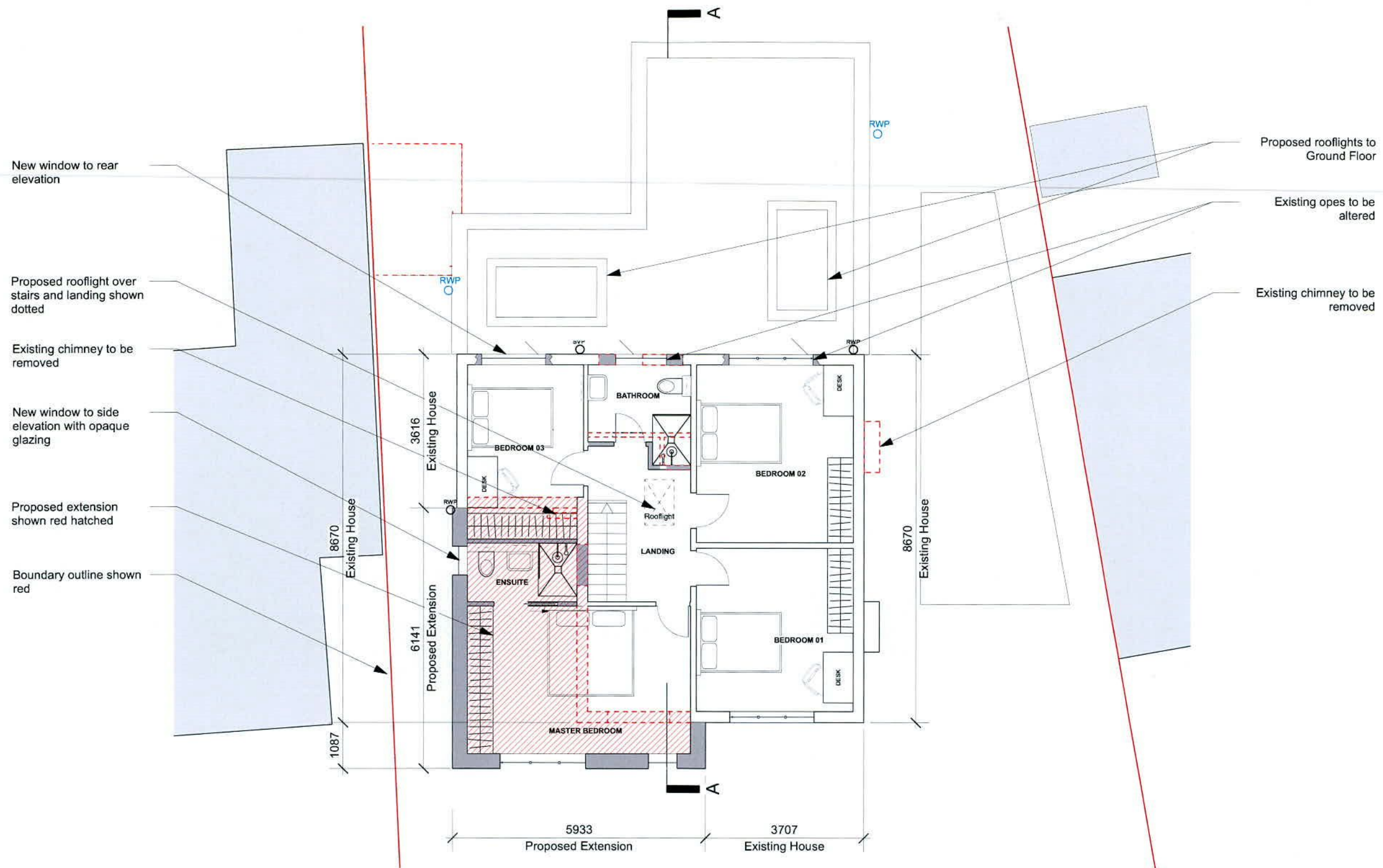
2 Proposed First Floor Plan Scale: 1:100
