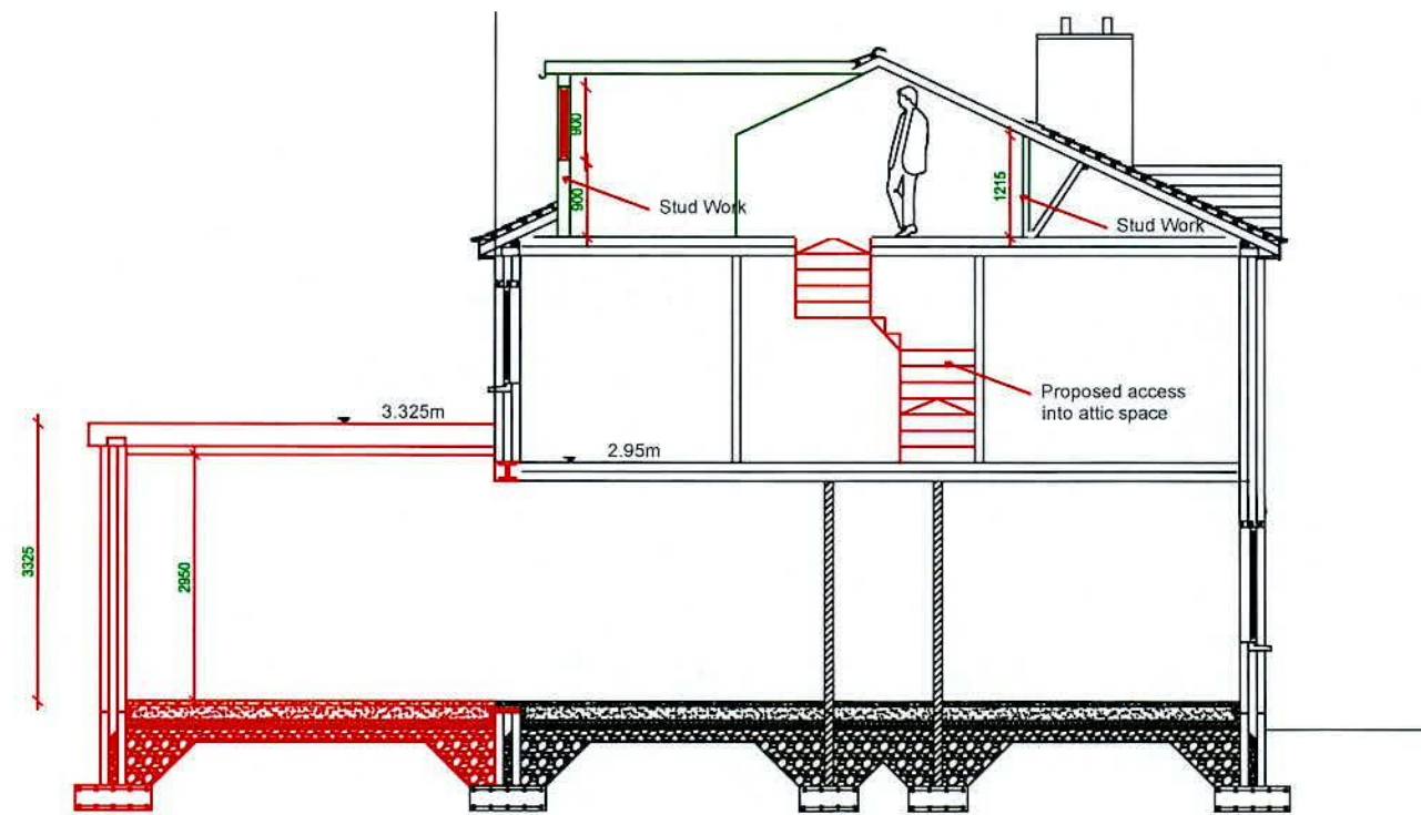
Proposed Section View
