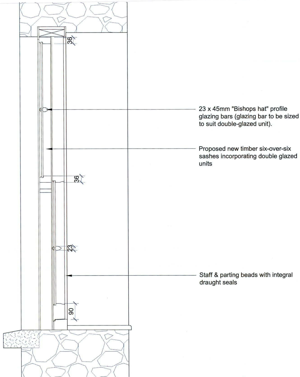
TYPICAL WINDOW SASH SECTION SCALE 1:10
