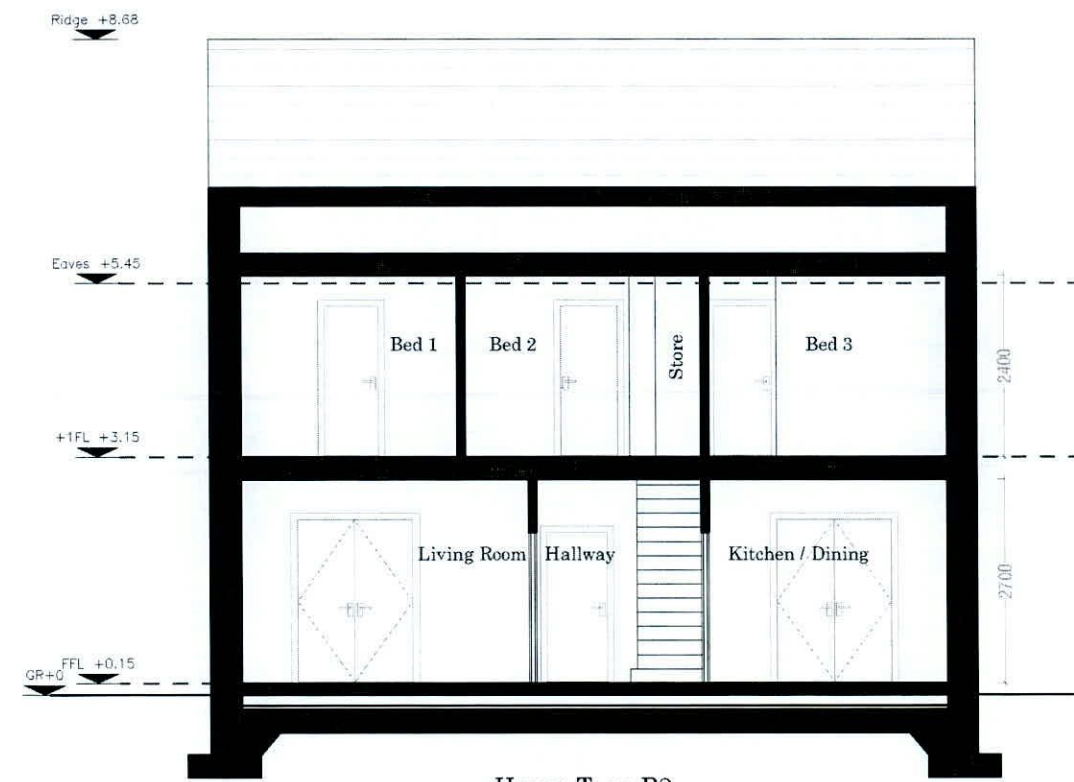
House Type B2 Section AA
