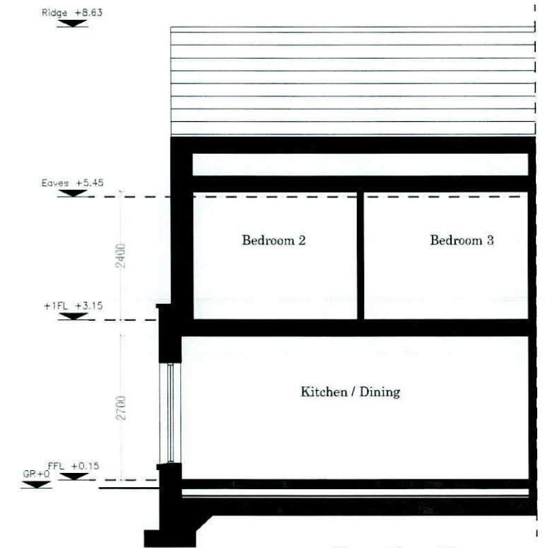
House Type A2 Section BB
