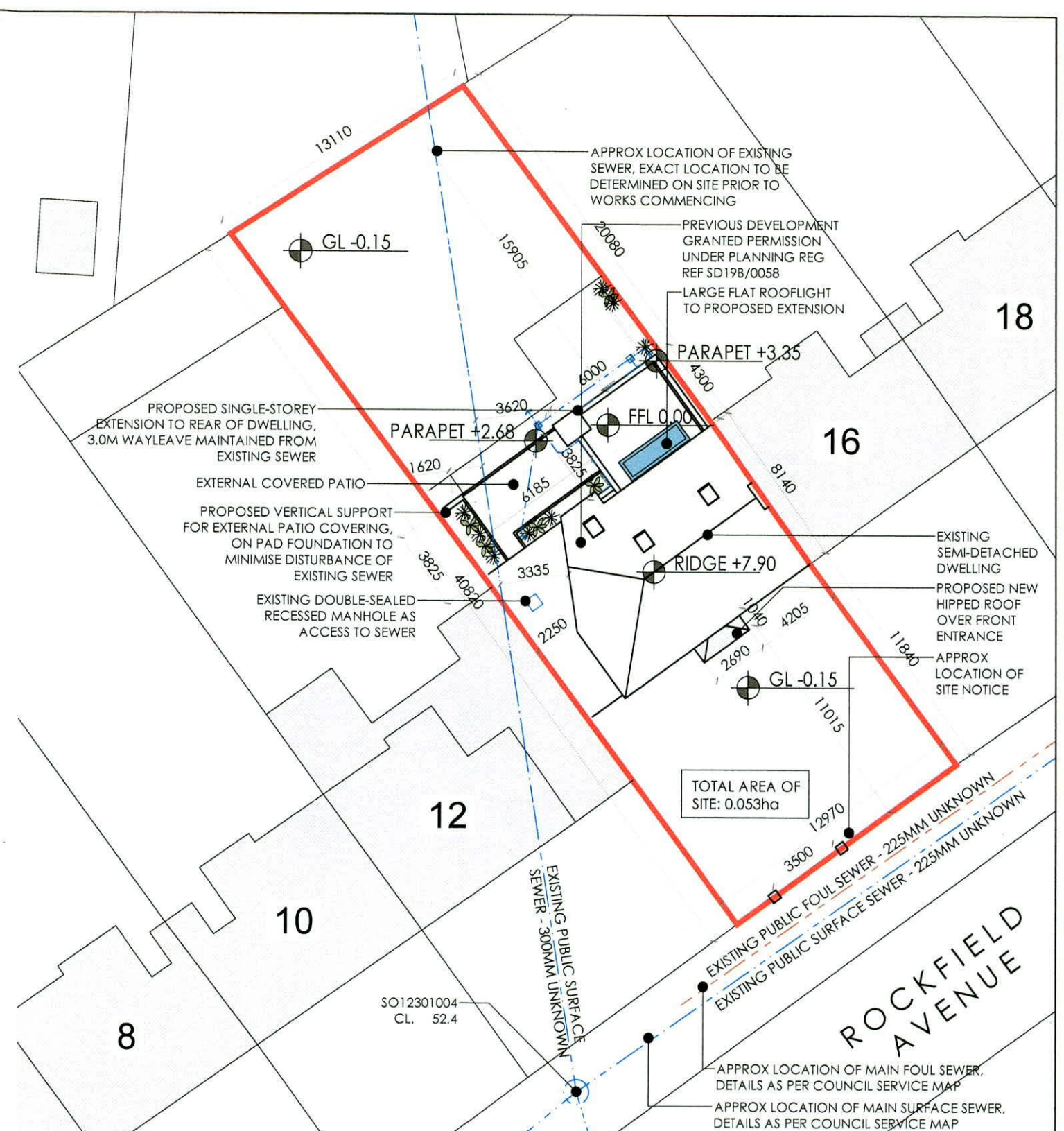
PROPOSED SITE LAYOUT MAP | LICENCE NO: 50267395 712034, 730069 scale 1:250 @ A3
