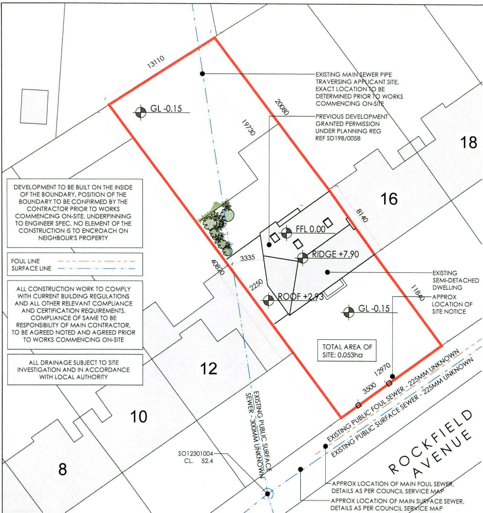
EXISTING SITE LAYOUT MAP | LICENCE NO: 50267395 712034, 730069 scale 1:250 @ A3
