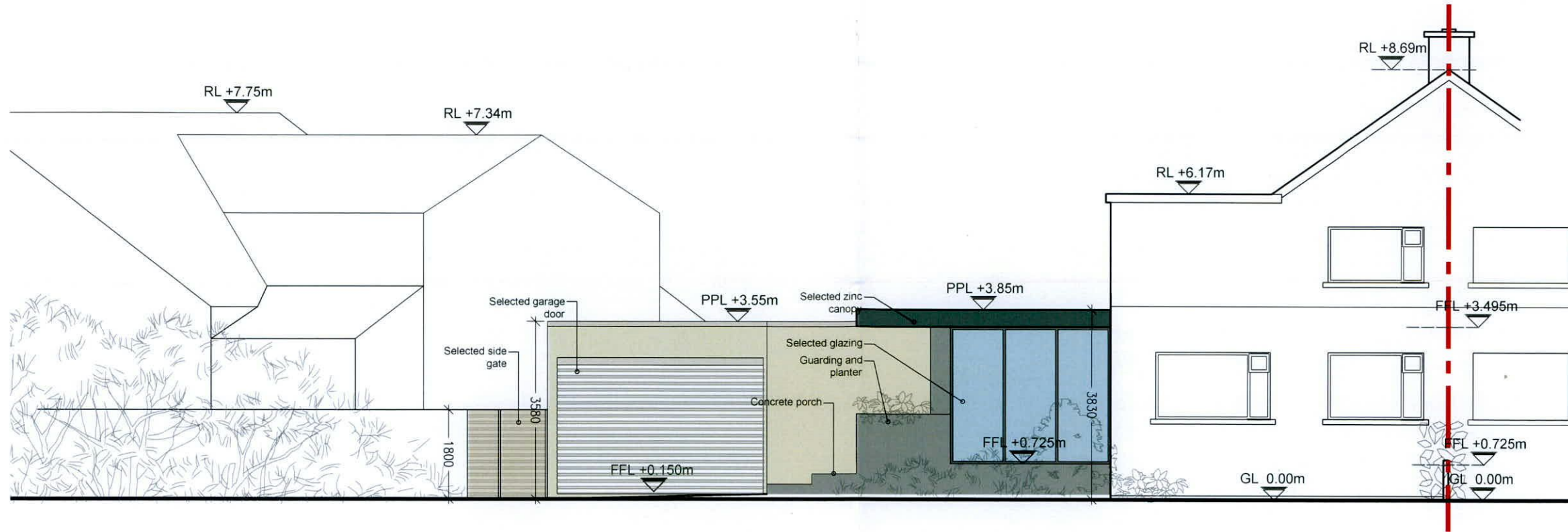
PROPOSED FRONT ELEVATION Scale 1:200
