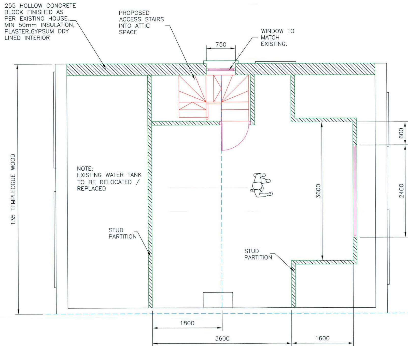
PROPOSED ATTIC FLOOR PLAN VIEW
