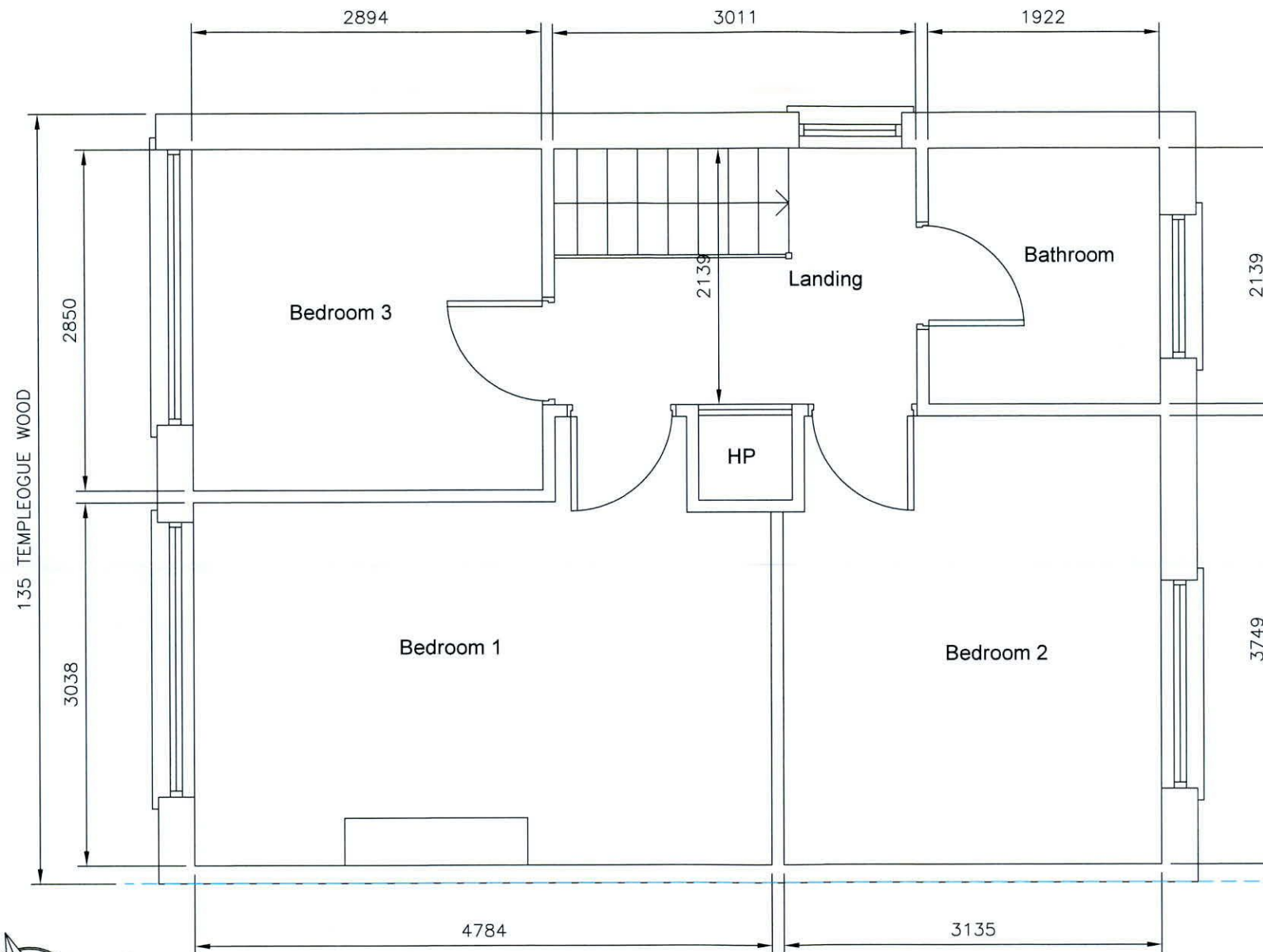
EXISTING FIRST FLOOR PLAN VIEW
