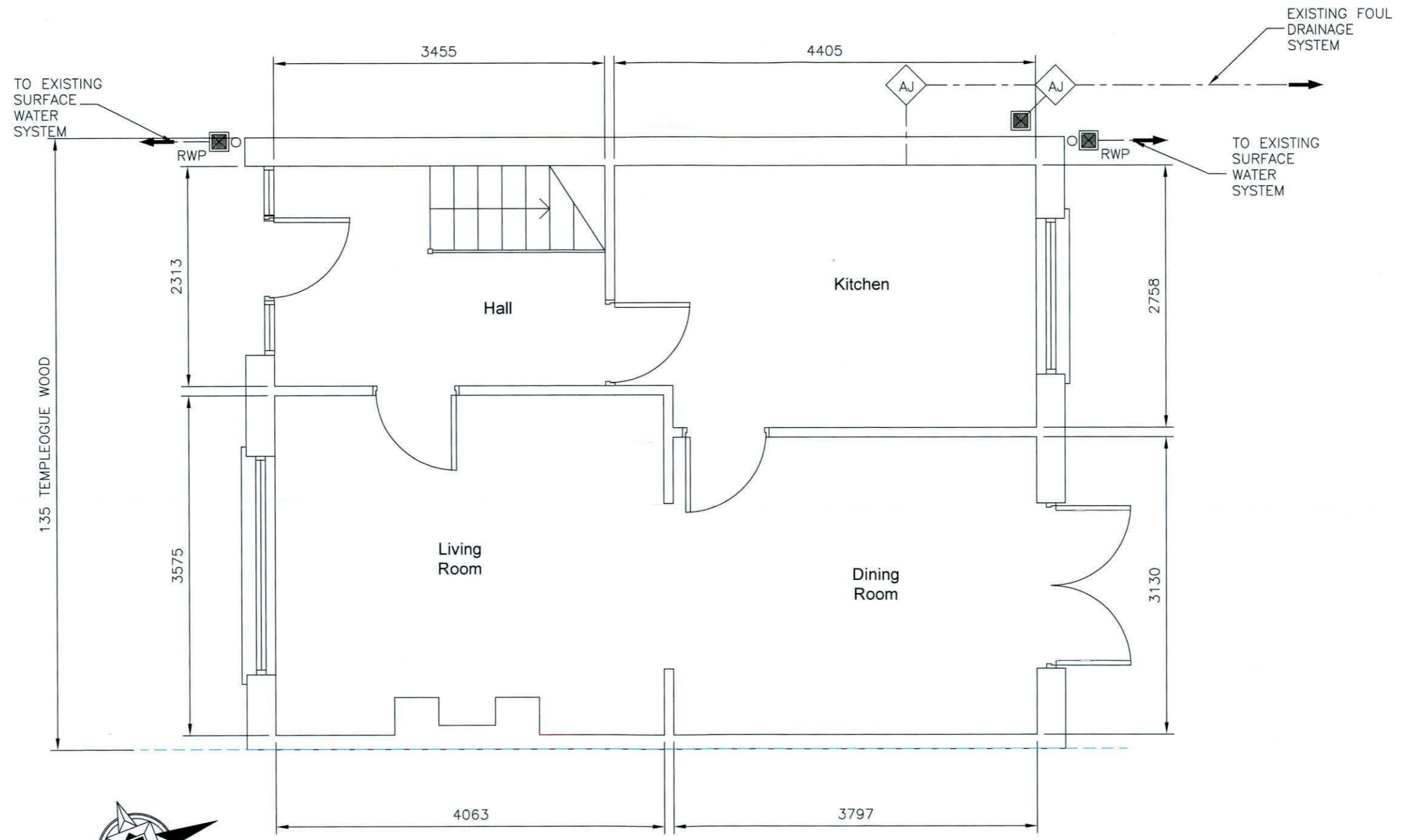
EXISTING GROUND FLOOR PLAN VIEW
