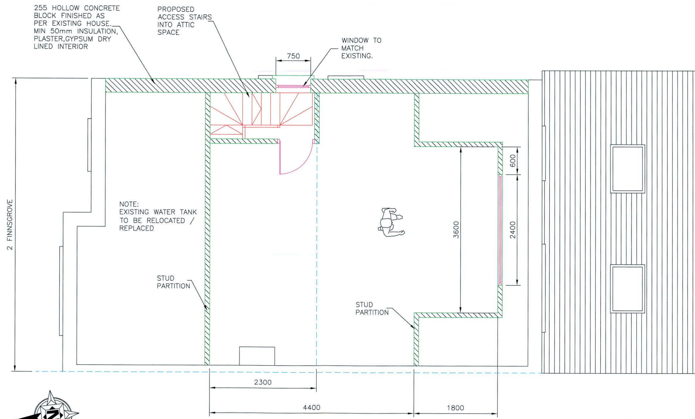
PROPOSED ATTIC FLOOR PLAN VIEW
