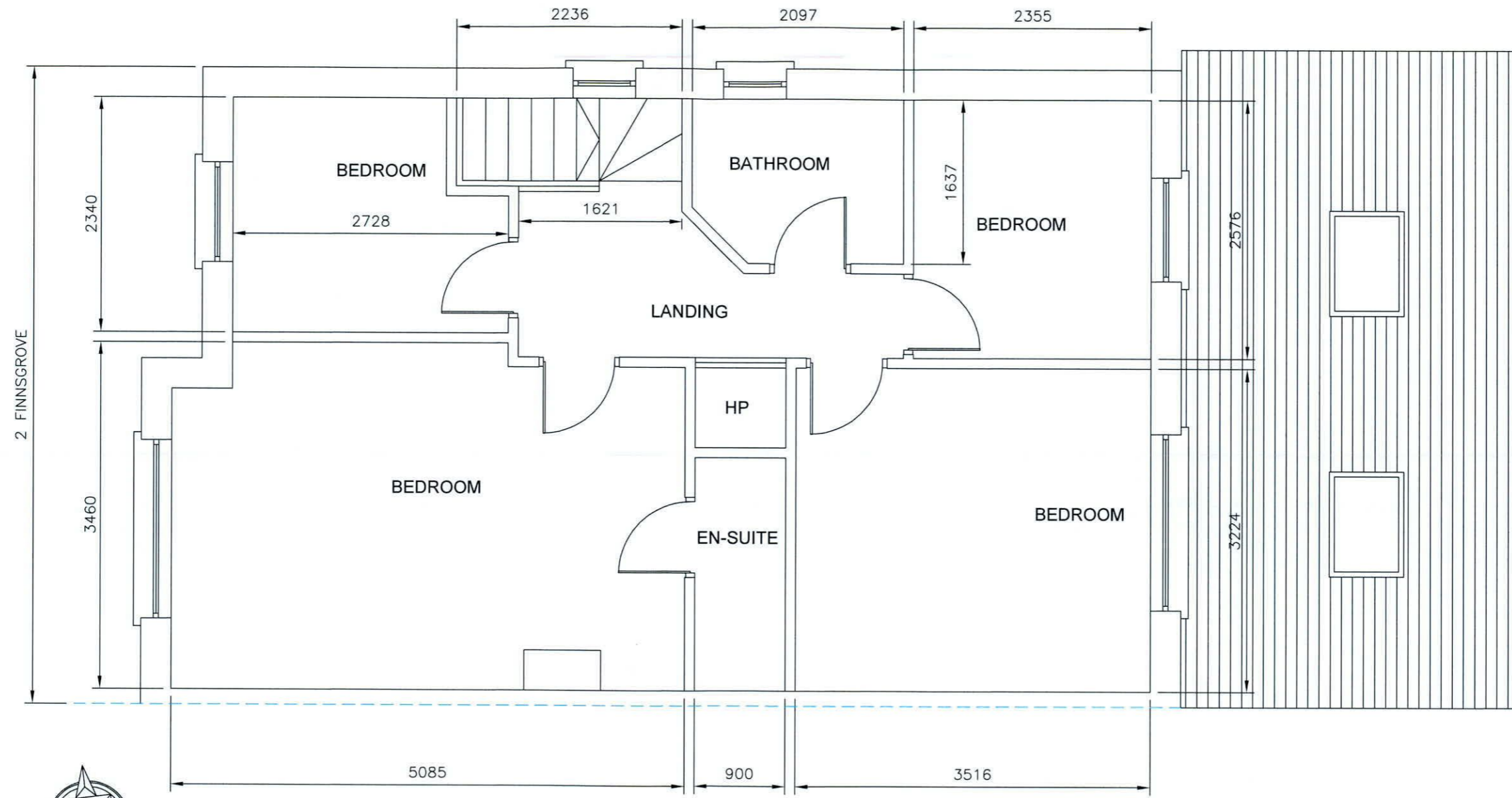
EXISTING FIRST FLOOR PLAN VIEW
