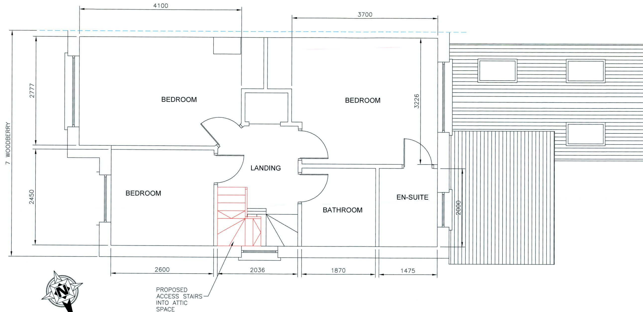
PROPOSED FIRST FLOOR PLAN VIEW
