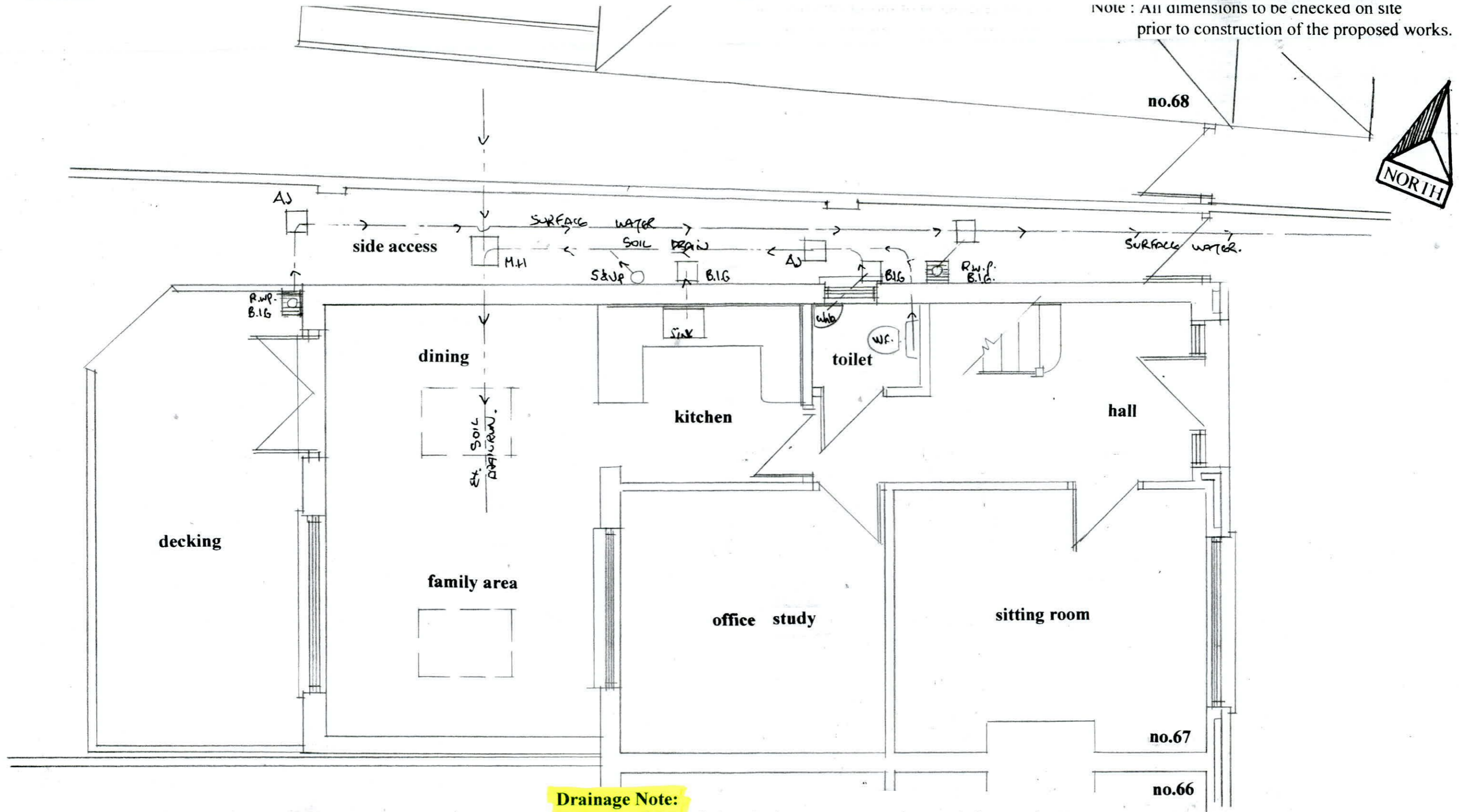
Proposed Drainage Layout scale 1:50.
