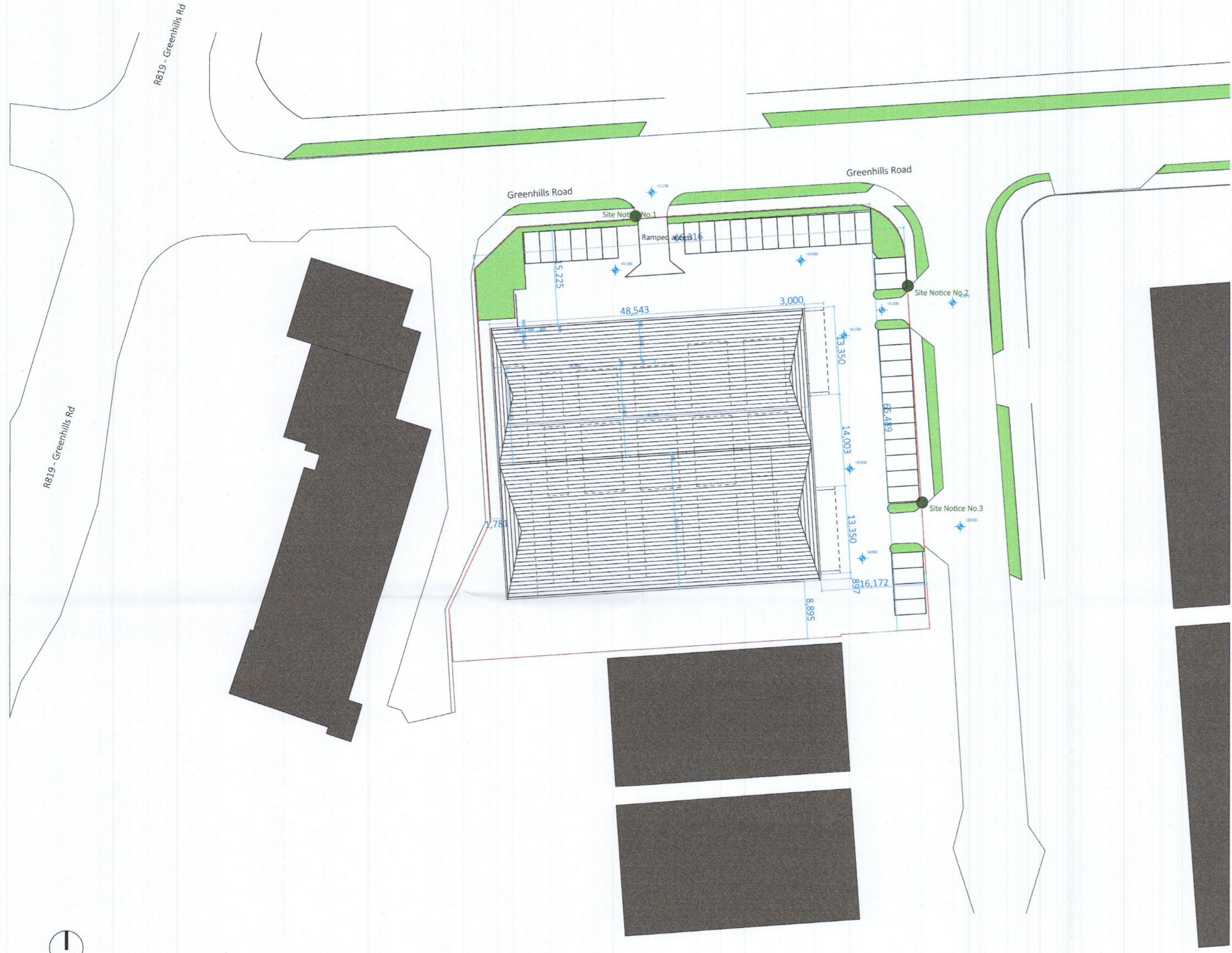
Existing Site Layout Scale 1:500
