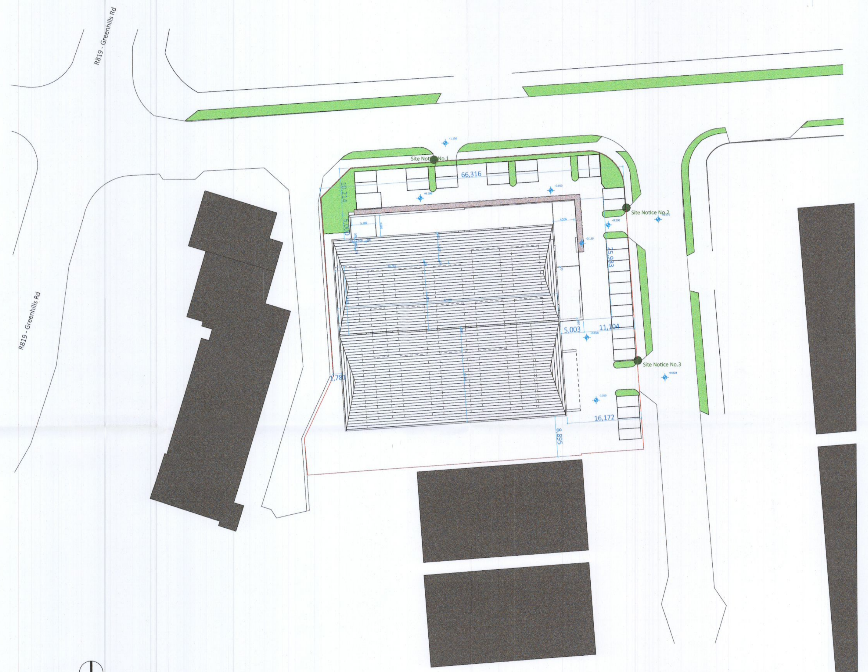
Proposed Site Layout Scale 1:500
