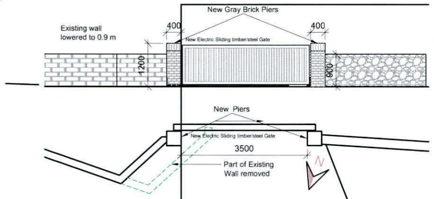
Proposed Access Gate Widening Scale 1:100@ A3
