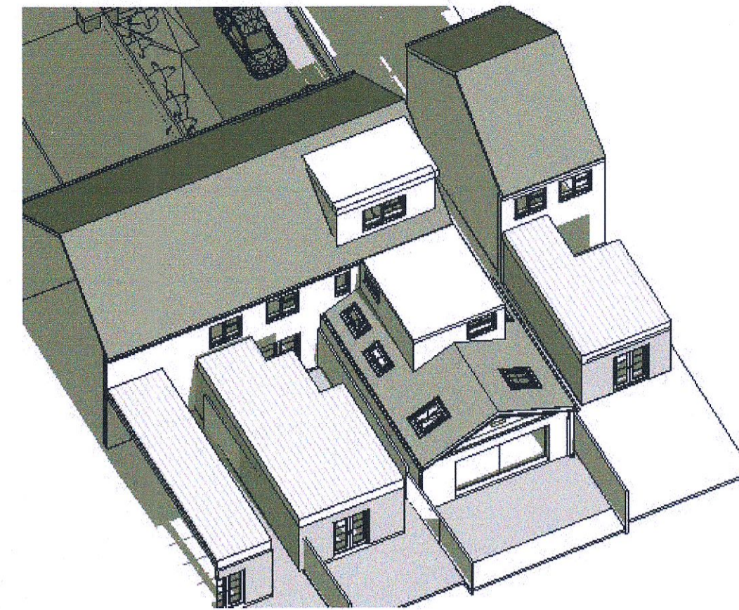
SPRING EQUINOX 4 PM
