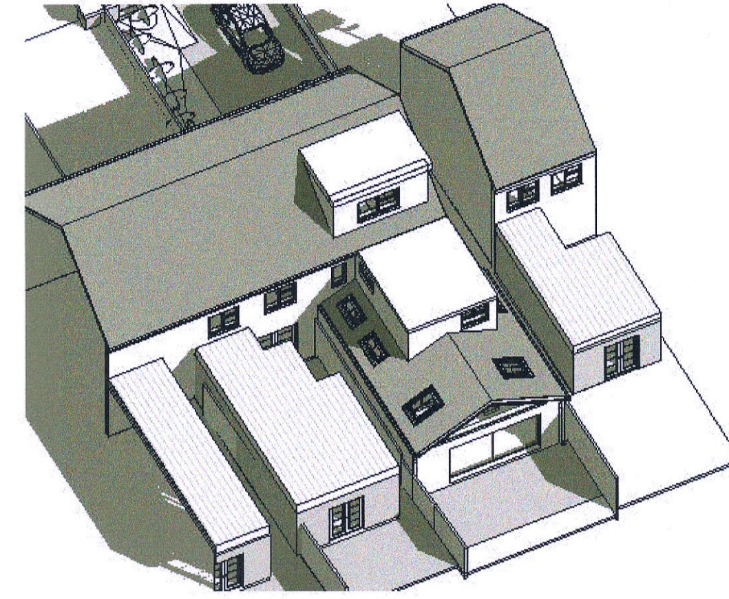
SUMMER SOLSTICE 2 PM
