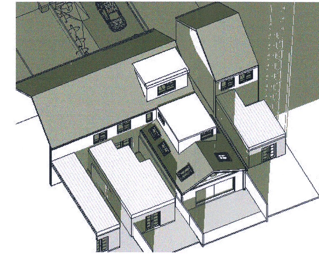
SPRING EQUINOX 7 PM
