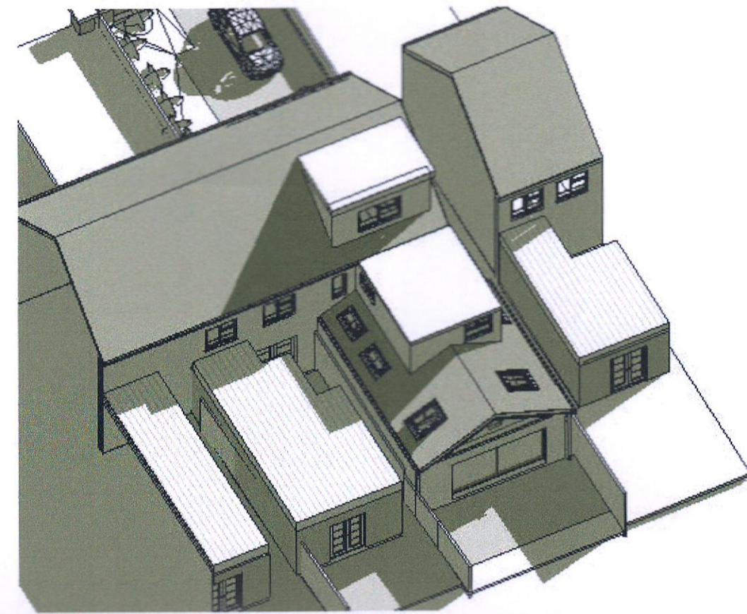
SUMMER SOLSTICE 10AM
