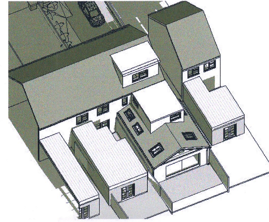
SUMMER SOLSTICE 4 PM
