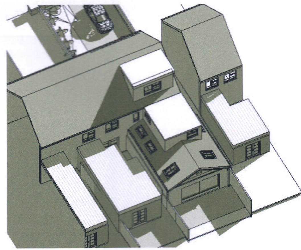
SPRING EQUINOX 10AM
