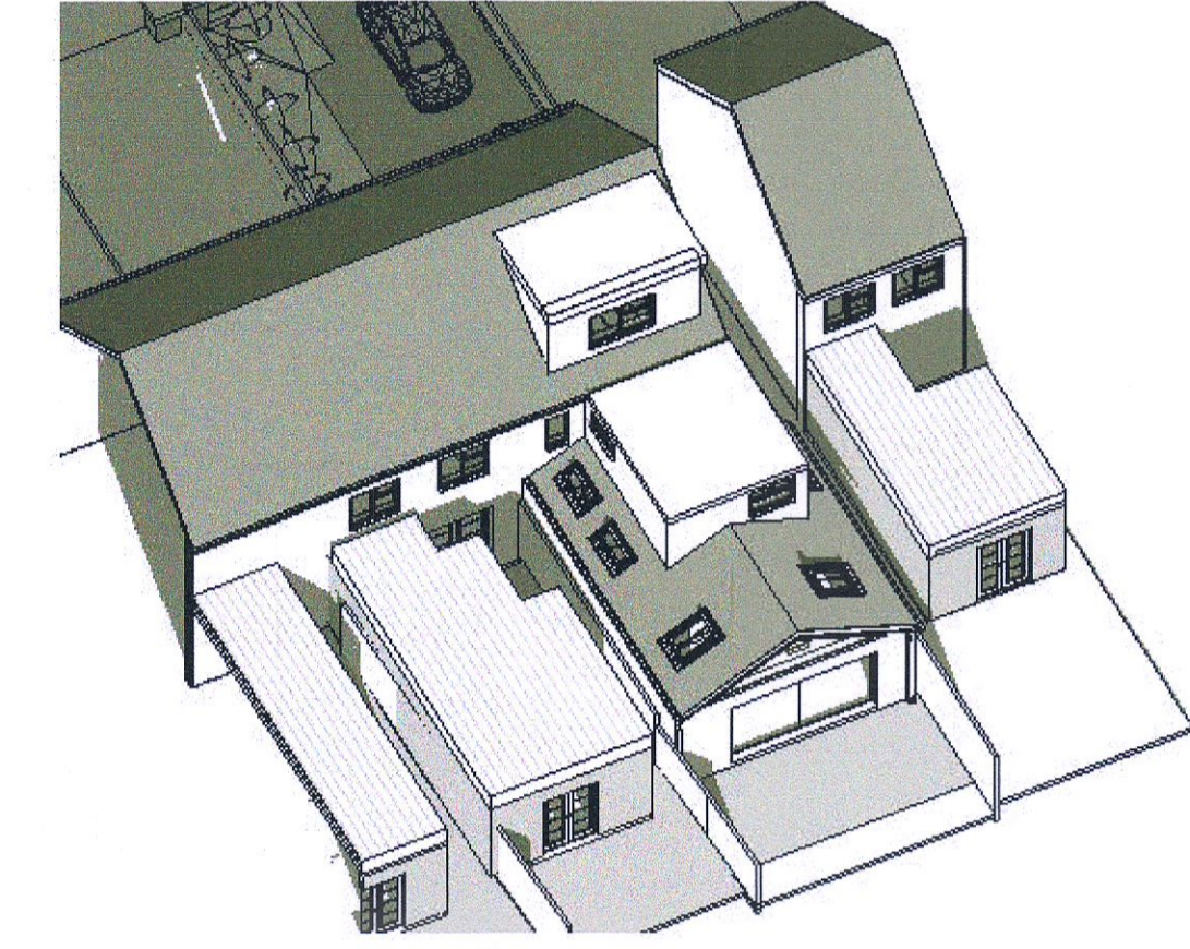
SUMMER SOLSTICE 7PM
