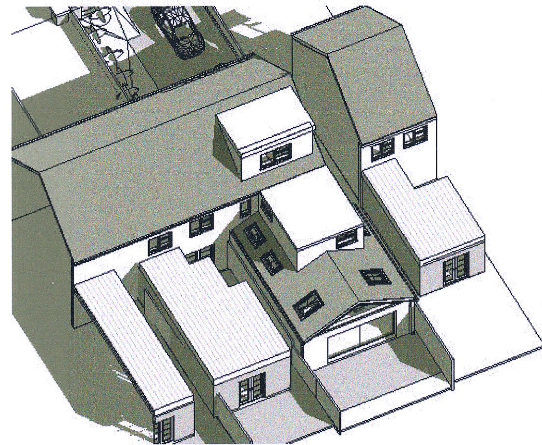
SPRING EQUINOX 2 PM
