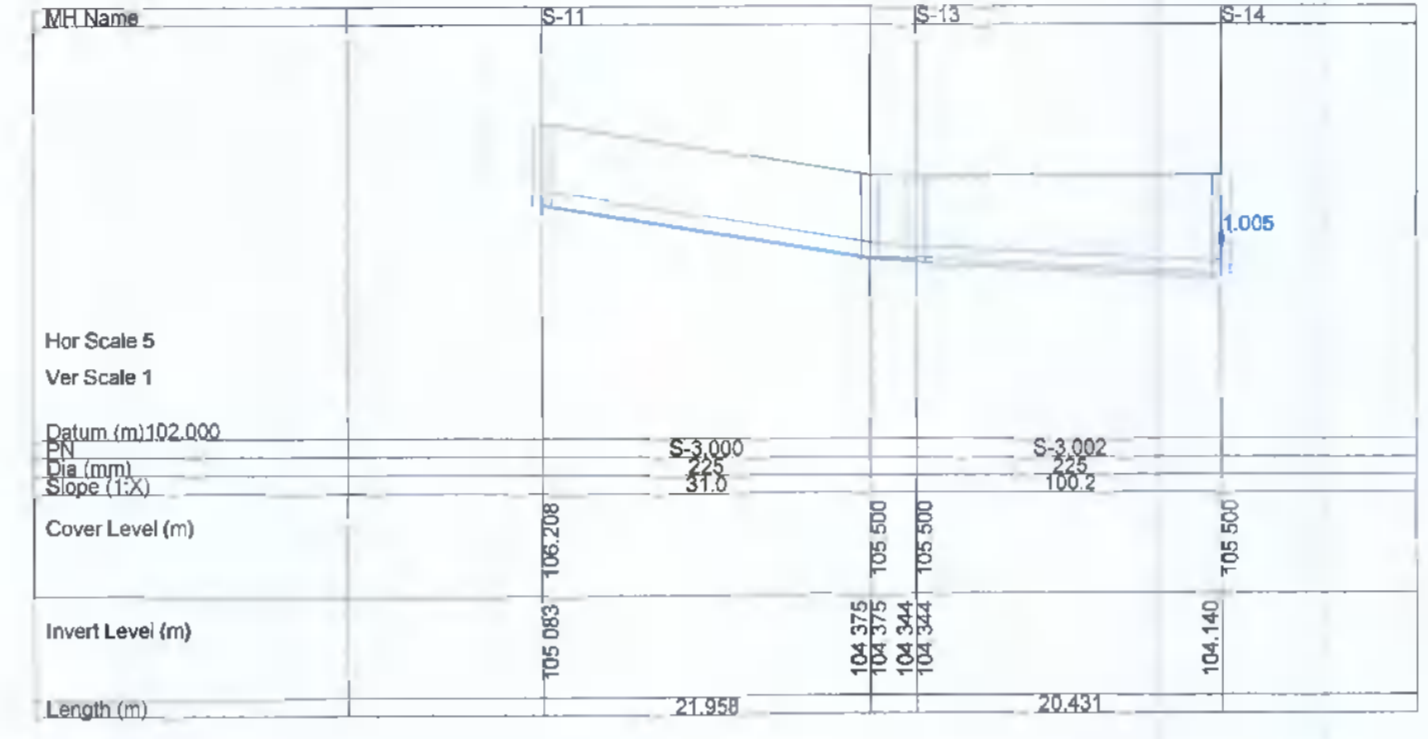
SURFACE WATER NETWORK: S3.000 - S3.002
