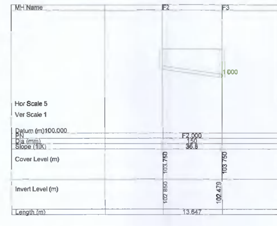
BASEMENT NETWORK: F2.000
