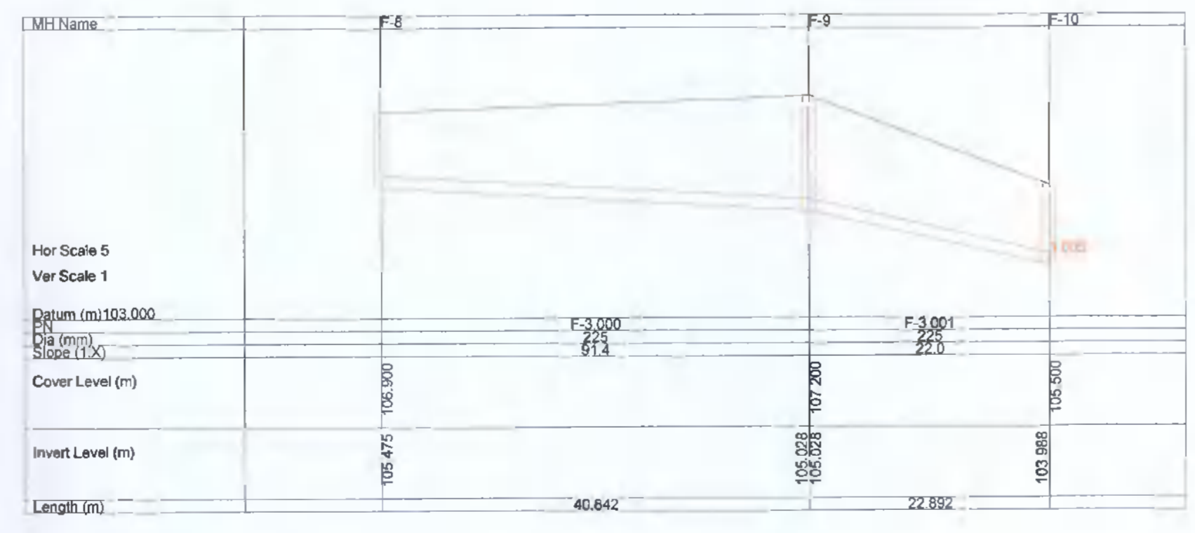
WASTEWATER NETWORK: F3.000 - F3.001
