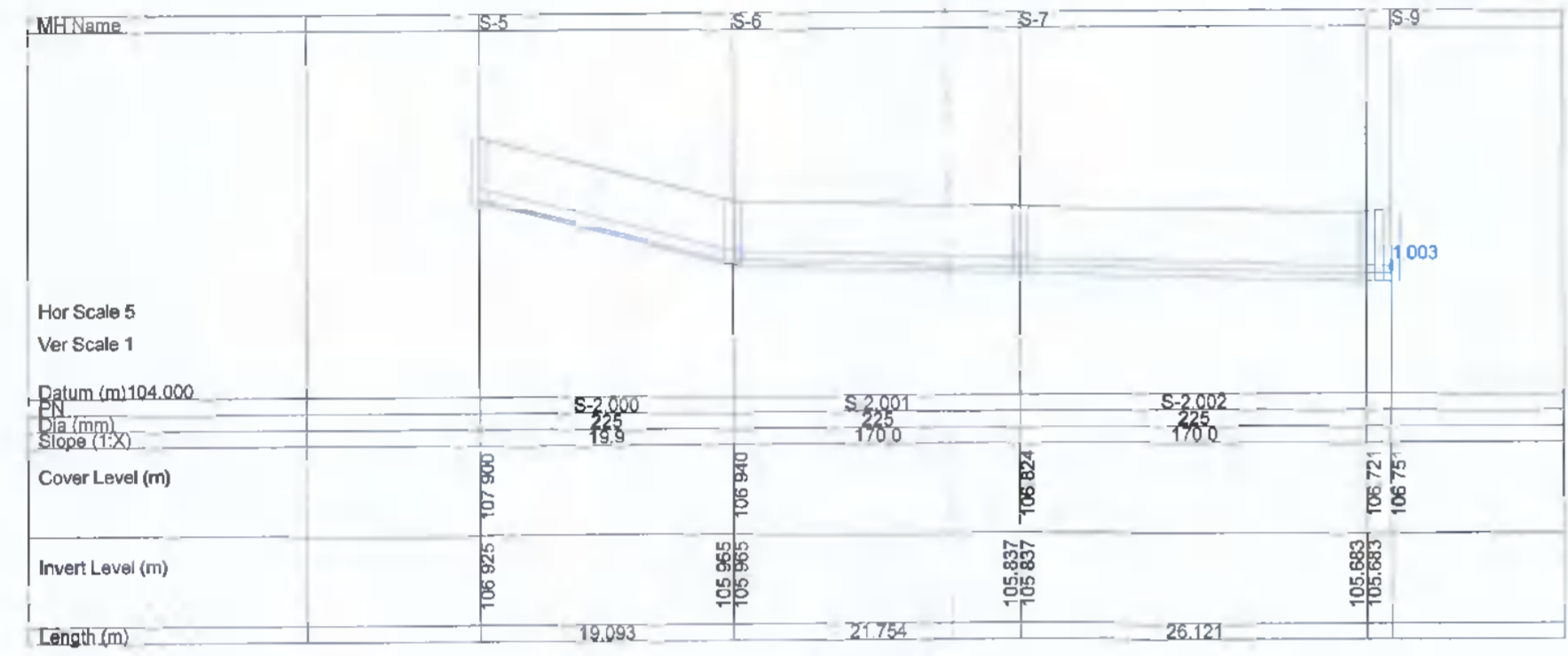
SURFACE WATER NETWORK: S2.000 - S2.002
