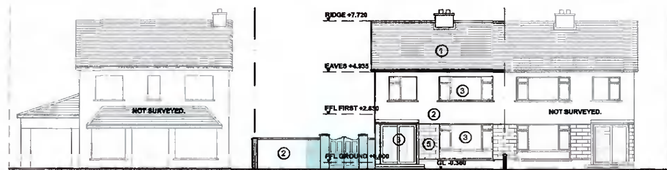
5 EXISTING CONTIGUOUS FRONT (SOUTH ELEVATION) PL04 SCALE 1:200
