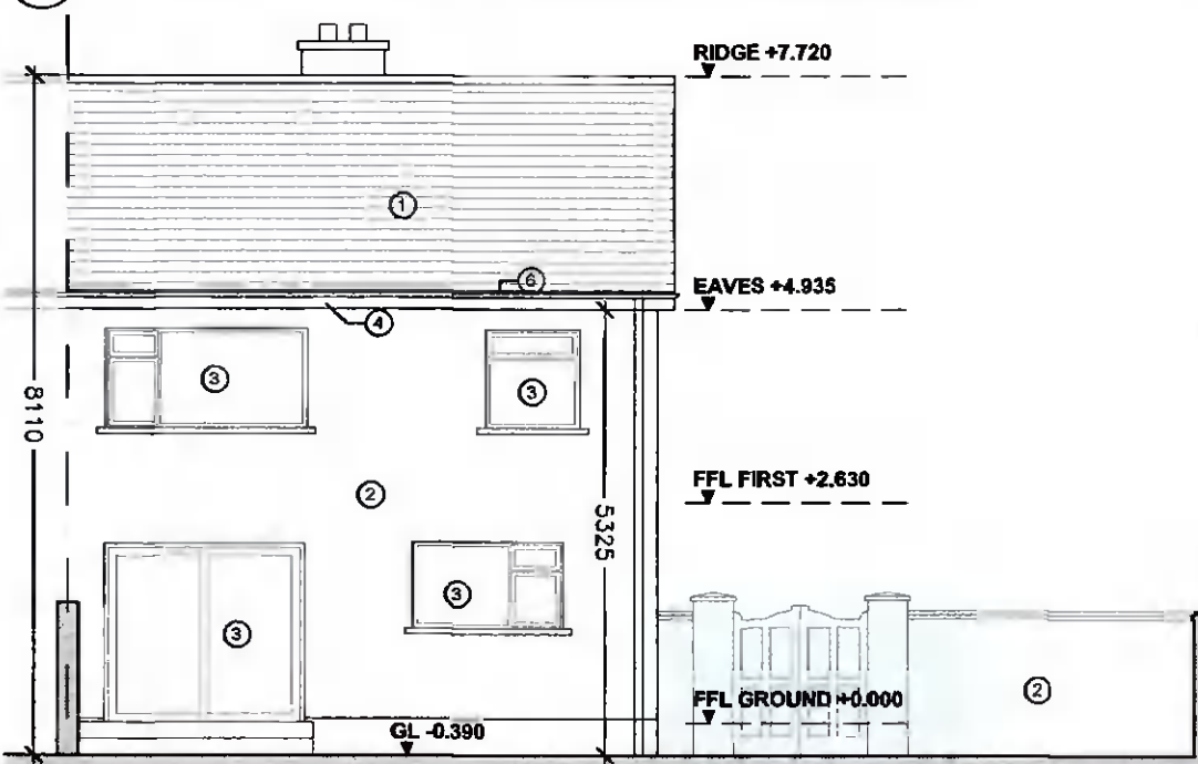
3 EXISTING REAR (NORTH) ELEVATION PL04 SCALE 1:100
