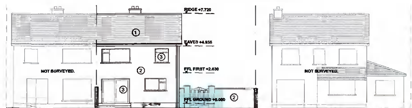
6 EXISTING CONTIGUOUS REAR (NORTH ELEVATION) PL04 SCALE 1:200
