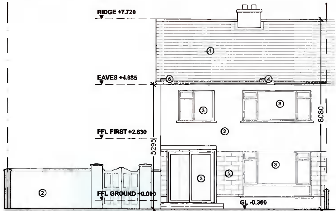
1 EXISTING FRONT (SOUTH) ELEVATION PL04 SCALE 1:100
