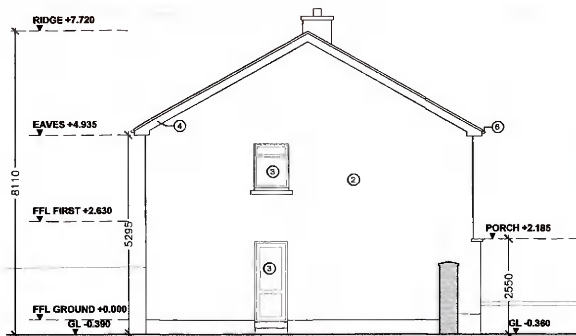
2 EXISTING SIDE (WEST) ELEVATION PL04 SCALE 1:100
