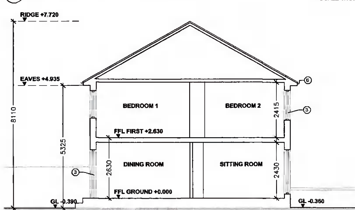
4 EXISTING SECTION A-A PL04 SCALE 1:100
