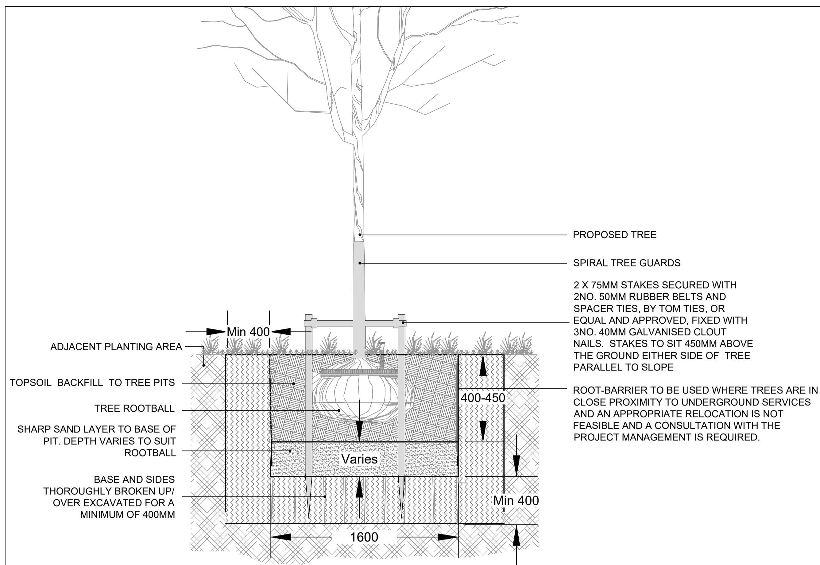
Tree Pit Detail scale 1:20 @A1
