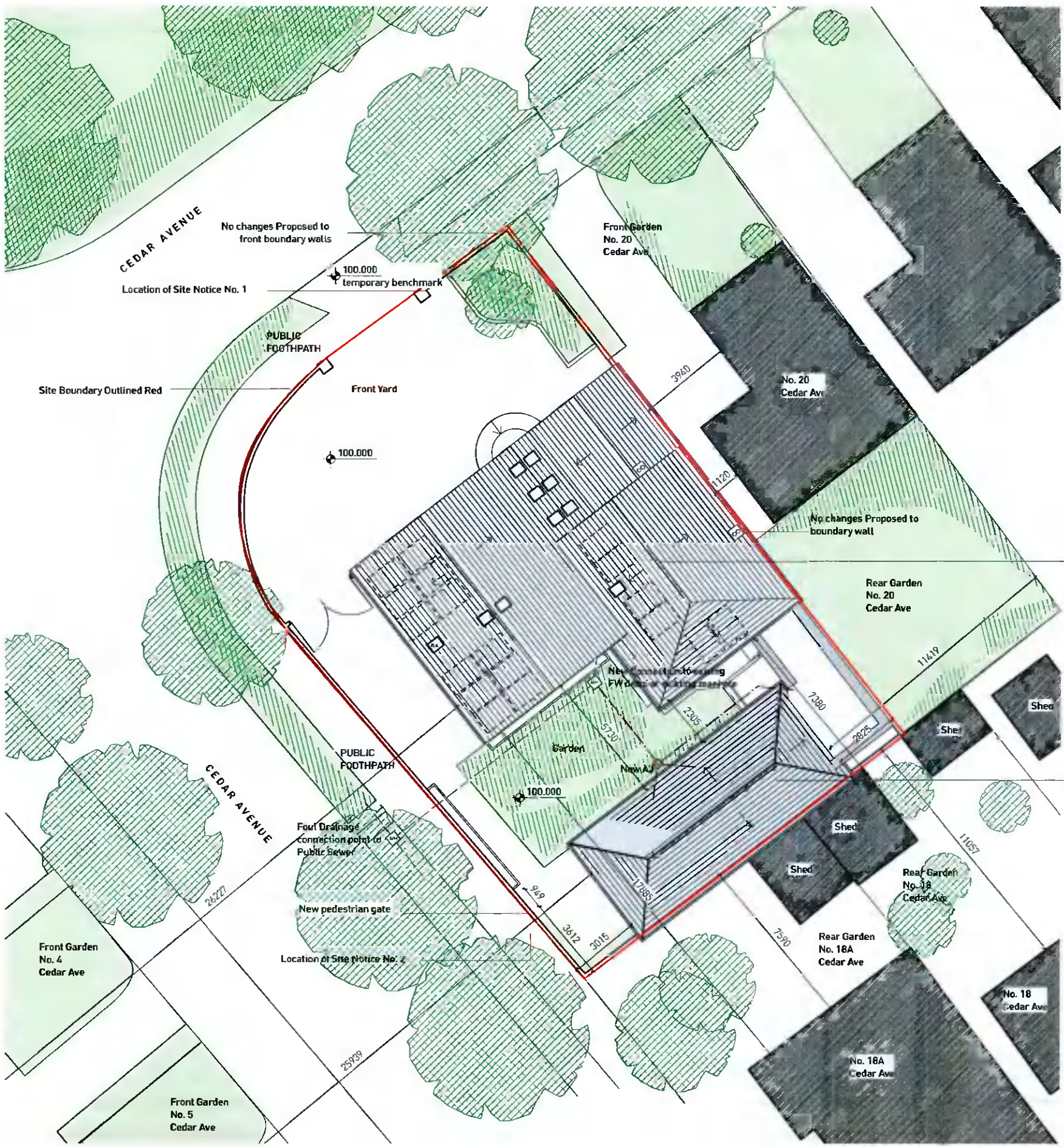
N PROPOSED SITE LAYOUT PLAN 1:200
