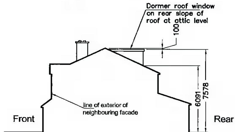
Proposed Dormer Side Elevation
