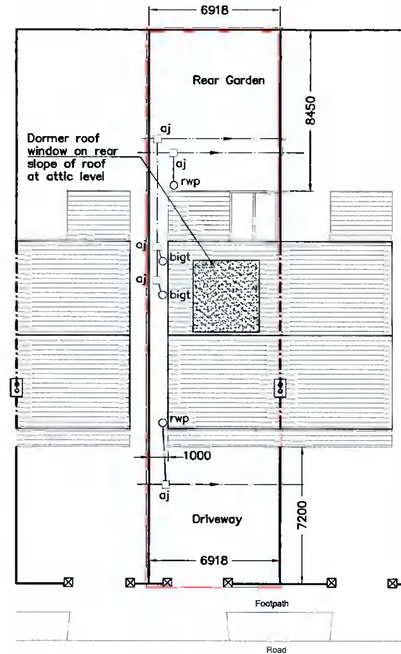
Proposed Block Plan & Drainage Layout SCALE 1:200
