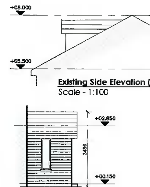
Existing Side Elevation (Porch) Scale - 1:100
