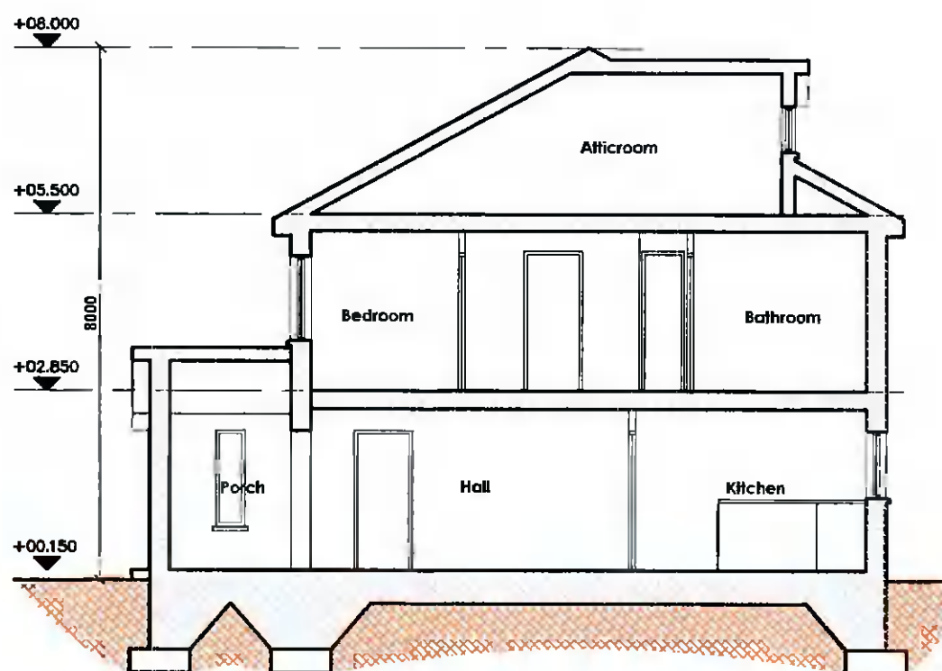
Existing Section A-A Scale - 1:100
