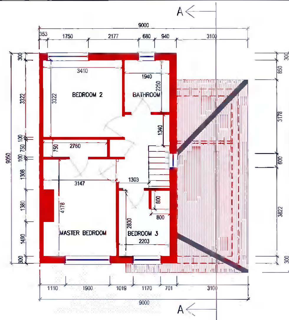
EXISTING FIRST FLOOR PLAN SHOWING ROOF OVER BEDROOM AND UTILITY ROOM.
